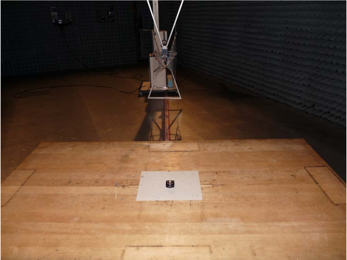
Photo 2: Test setup for radiated measurements, 30 MHz – 1 GHz
