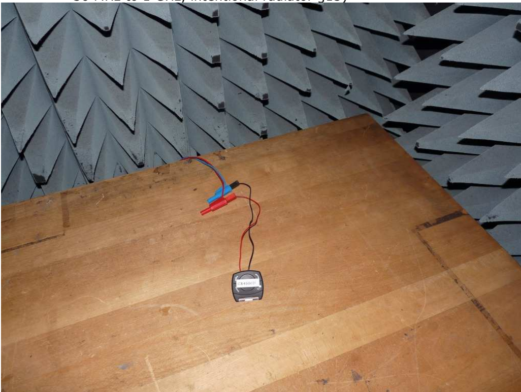
Photo 2: Test Setup for radiated measurement H-Field
