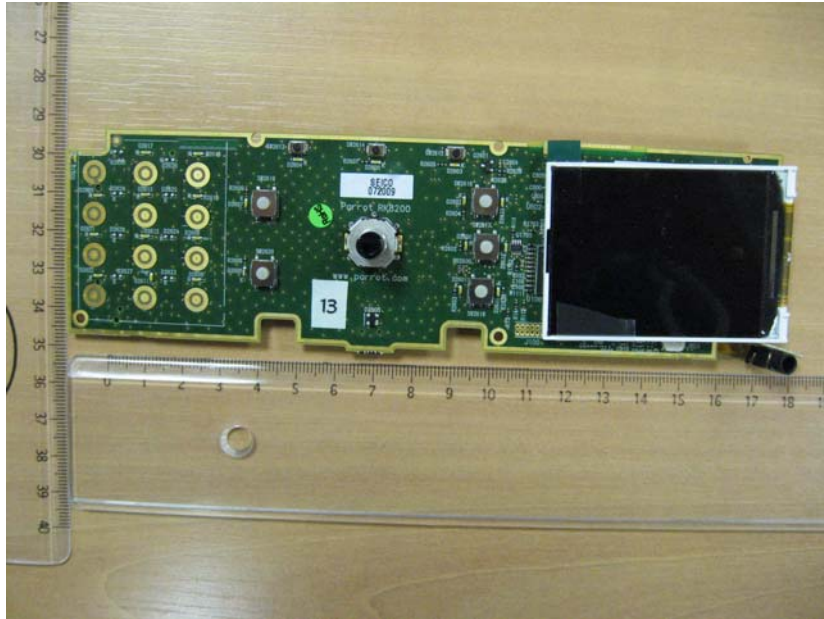
Front panel (Top View)
