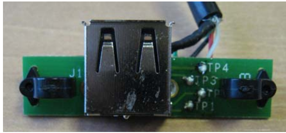
PARELIA USB BOARD (Top)
