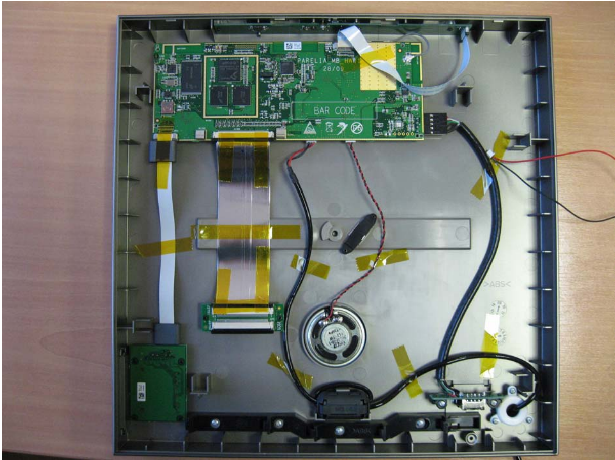
PARELIA: Position of boards
