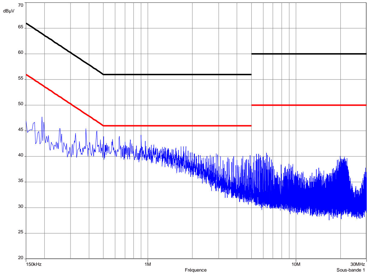
Peak measurement on the neutral
