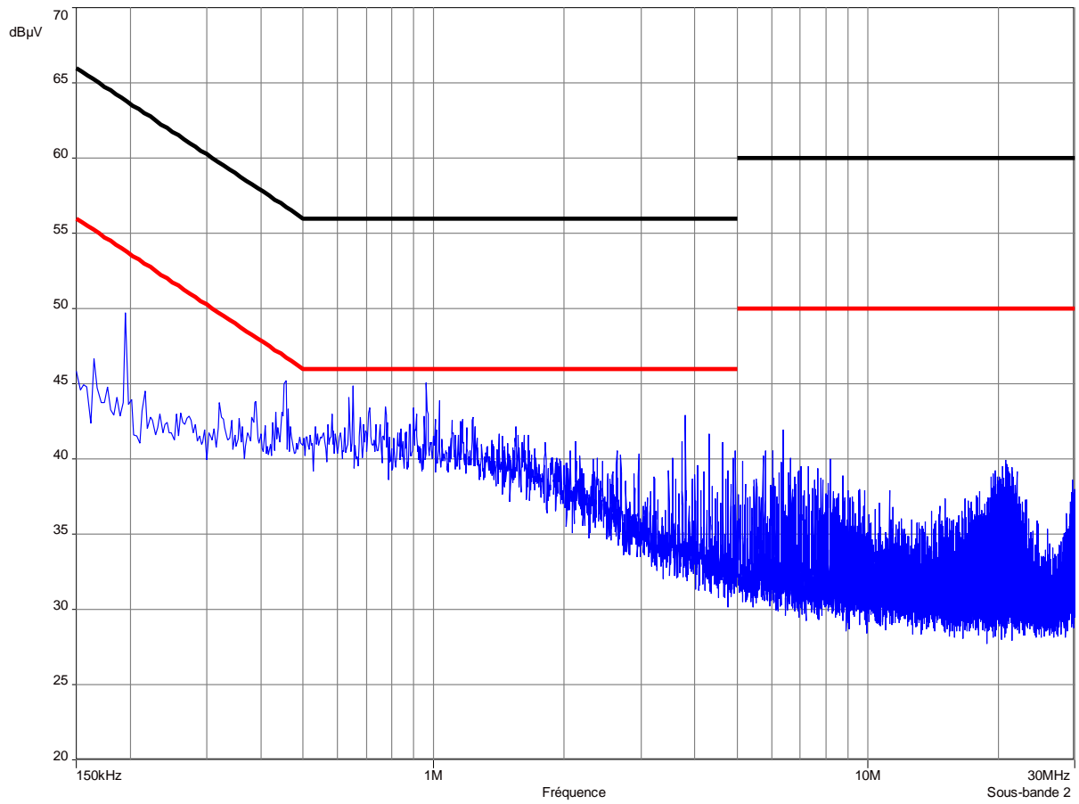
Peak measurement on the line
