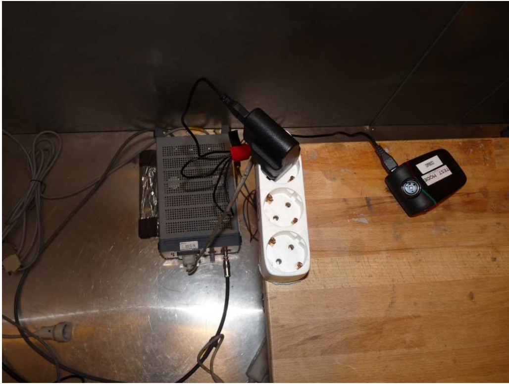
Photo 4: Test setup for conducted measurements, AC Mains
