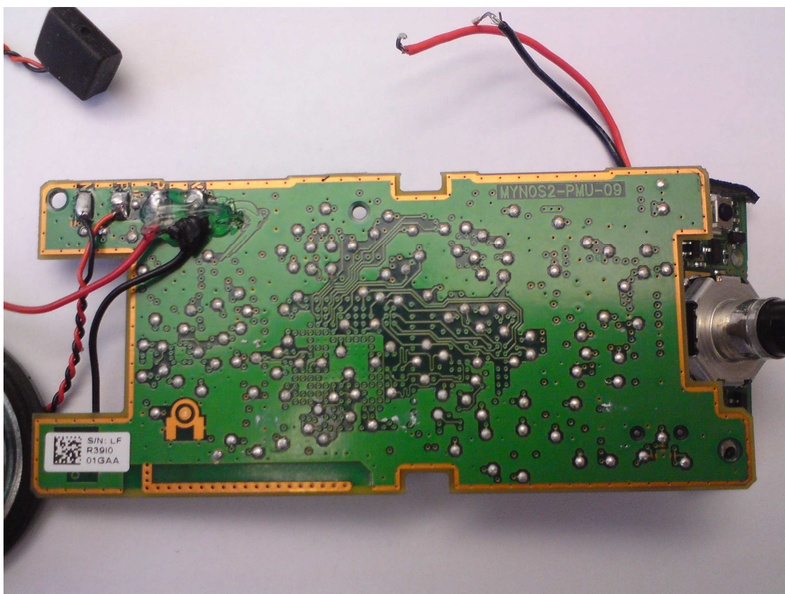
Mainboard (bottom view) with Daughterboard connected
