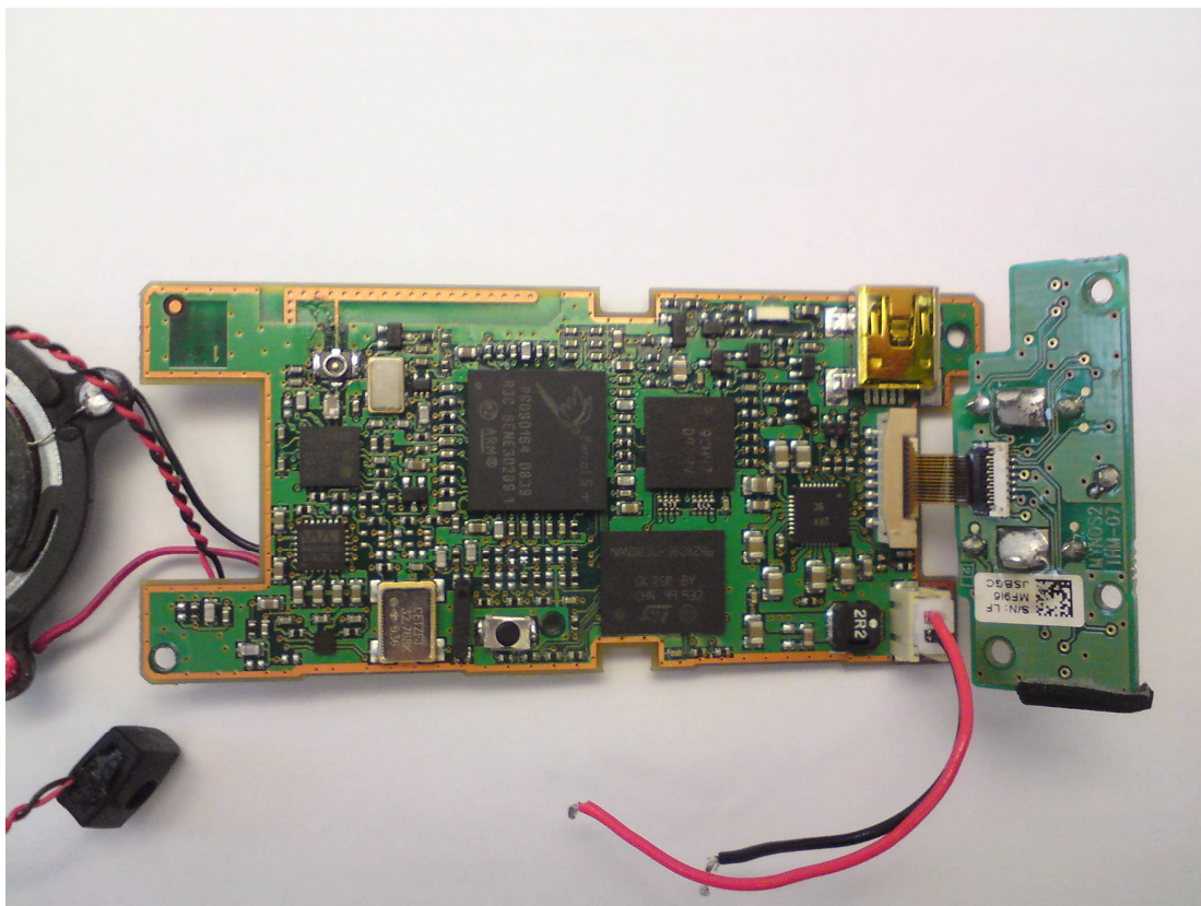
Mainboard (top view) with Daughterboard connected
