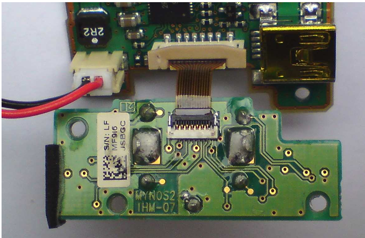
Daughterboard (bottom view)
