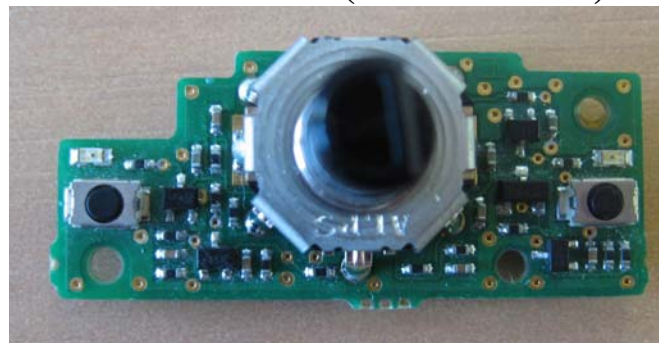
Daughter Board (Top View)
