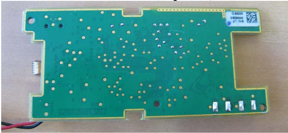
Mother Board (Bottom View)
