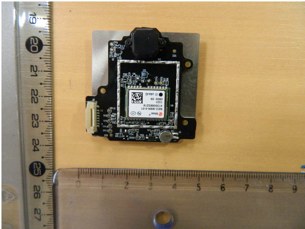
GNSS board(Top)
