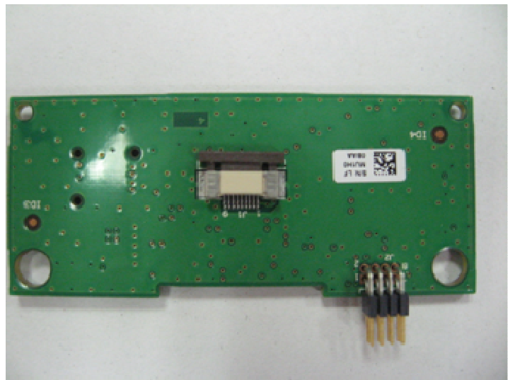
NAV Board (Bottom)
