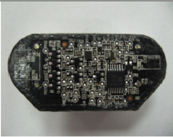
US Board (Top)
