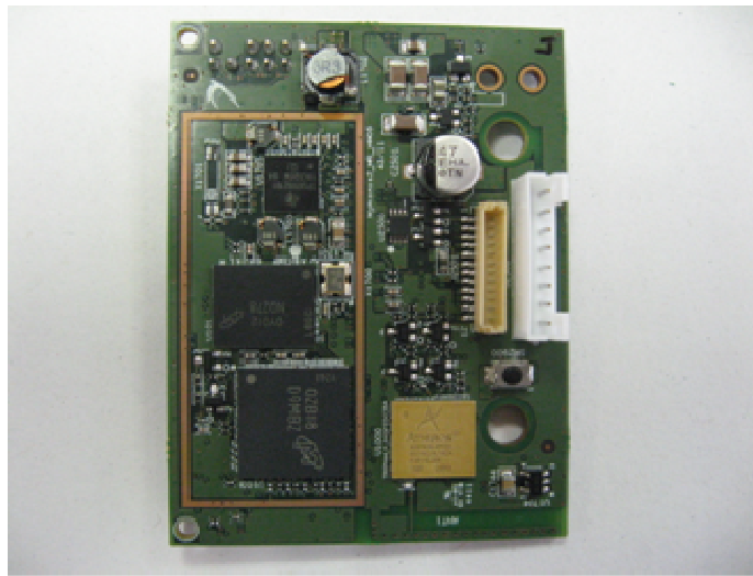
Mother board without shielding
