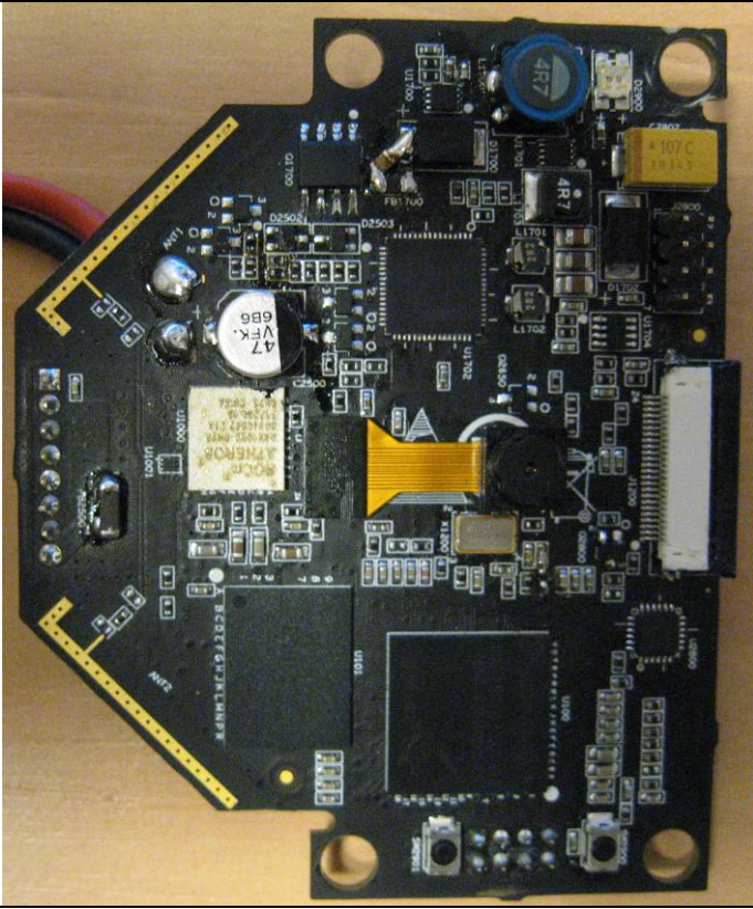
Mother Board (Top)
