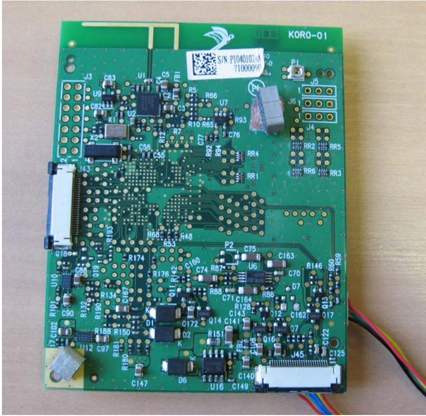
Mother Board (Top)
