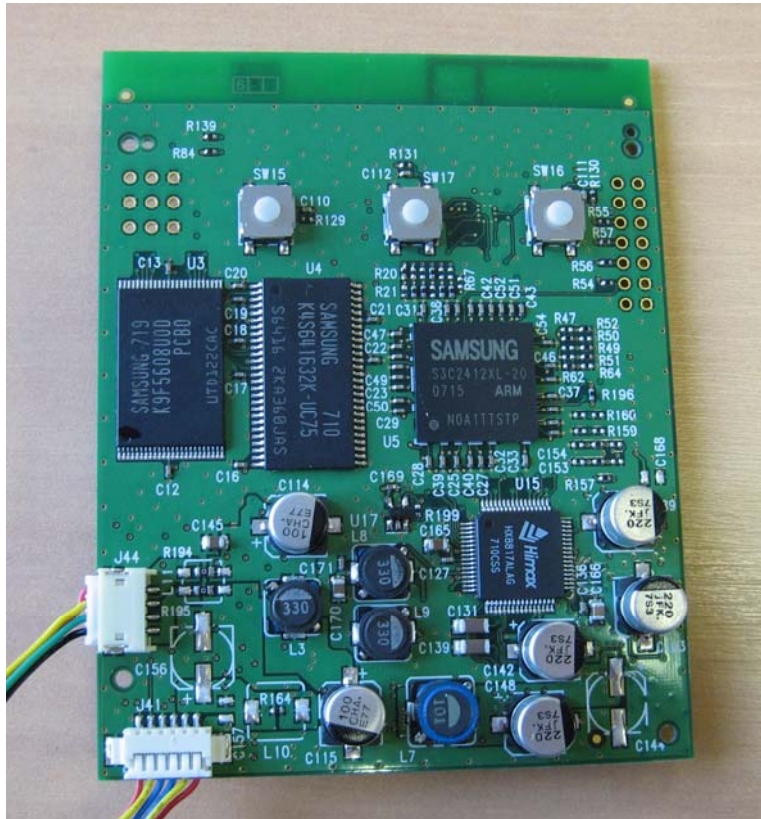
Mother Board (Bottom)
