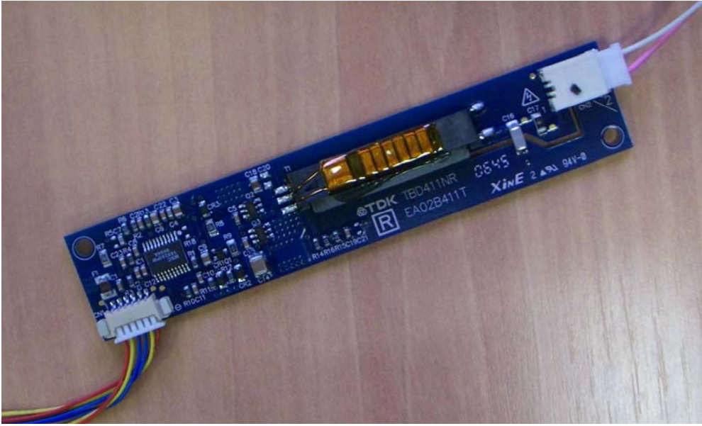
Inverter (Top)
