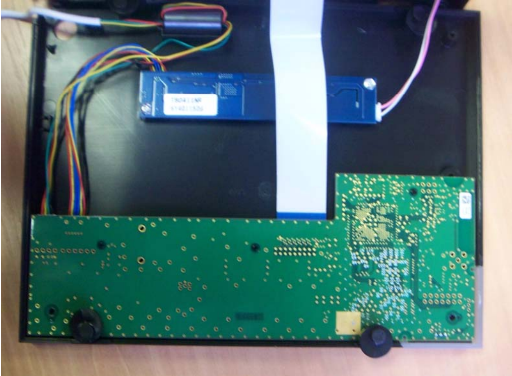
Mother Board and Inverter (Bottom)
