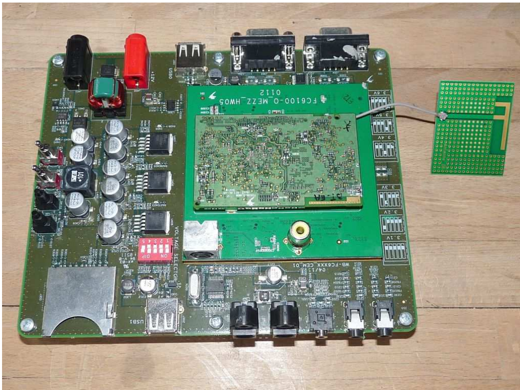
Photo 5: FC6100 module with the external F-antenna
