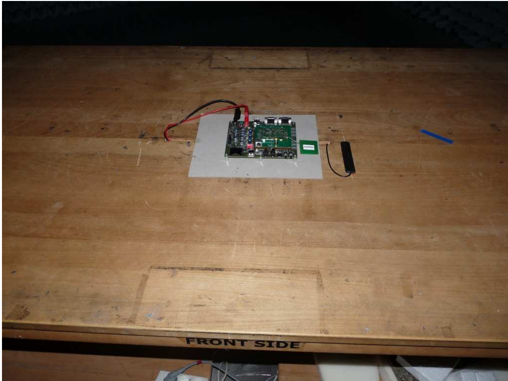
Photo 4: Test setup for radiated measurements (30 MHz to 1 GHz), FCC 15.247 Module with external Antenna
