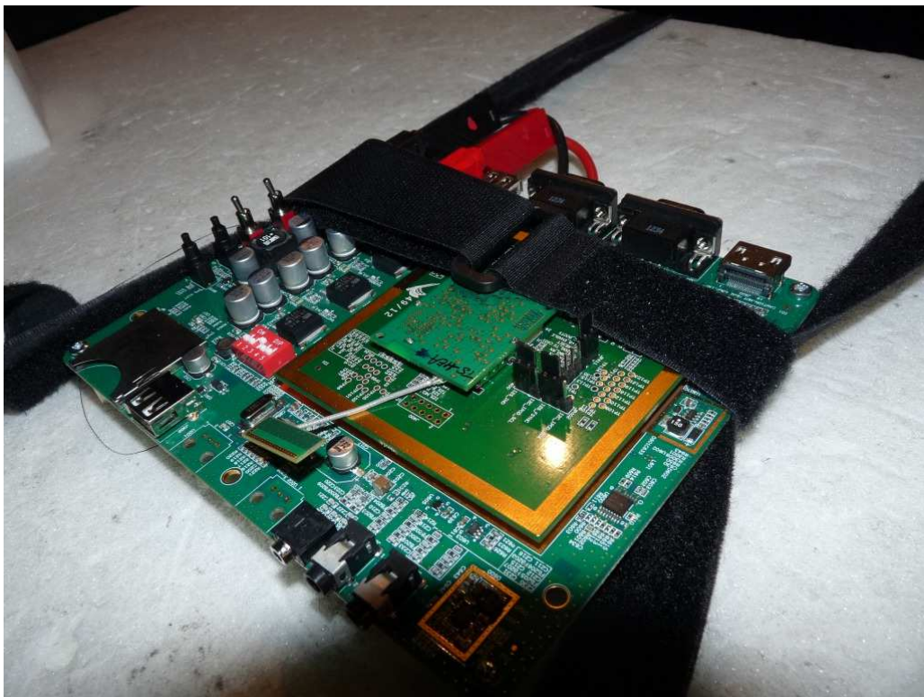
Photo 5: FC6000TS module with the external antenna
