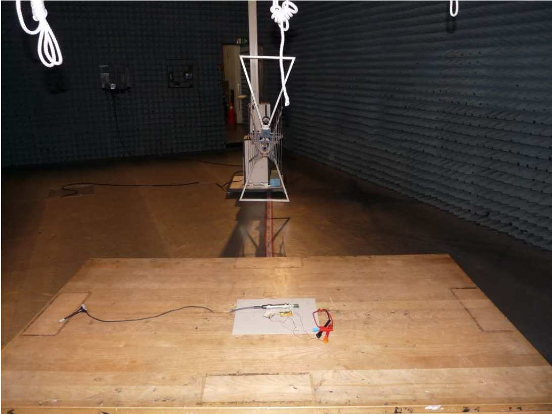
Photo 1: Test setup for radiated measurements (30 MHz to 1 GHz)
