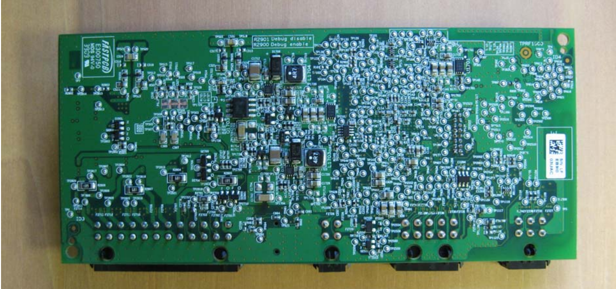
eBox4R2 (BOTTOM)
