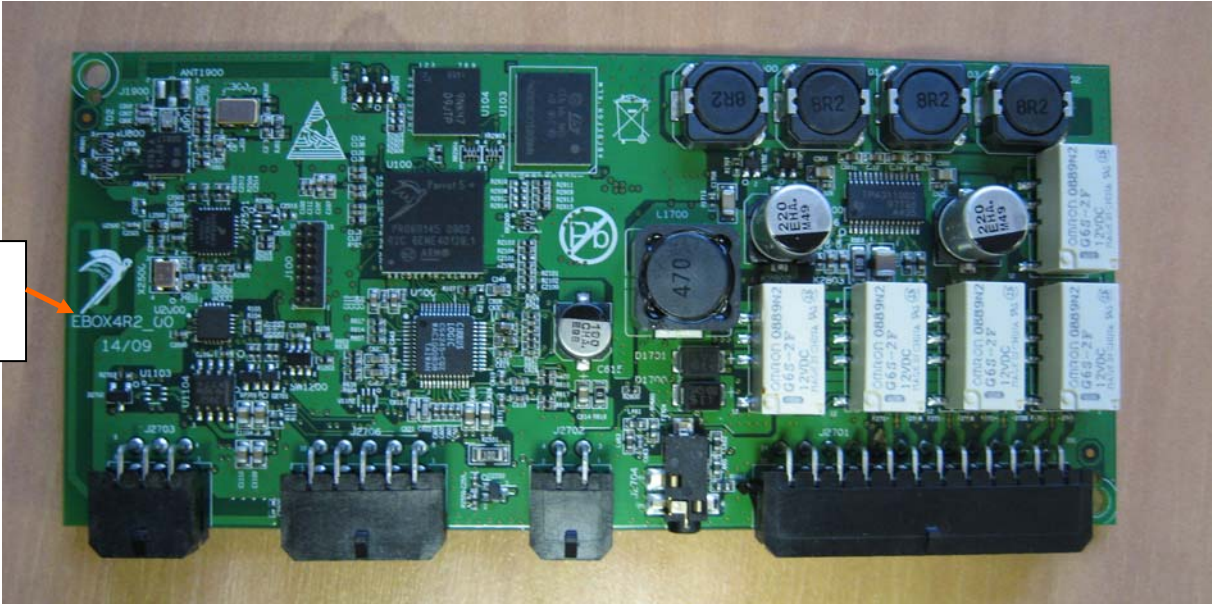
eBox4R2 (TOP)
