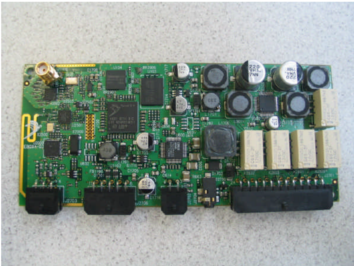
Photo 6: EUT (PCB, without housing, with temporary antenna connector)
