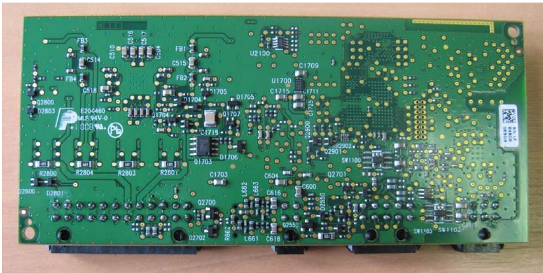
E-BOX (BOTTOM)
