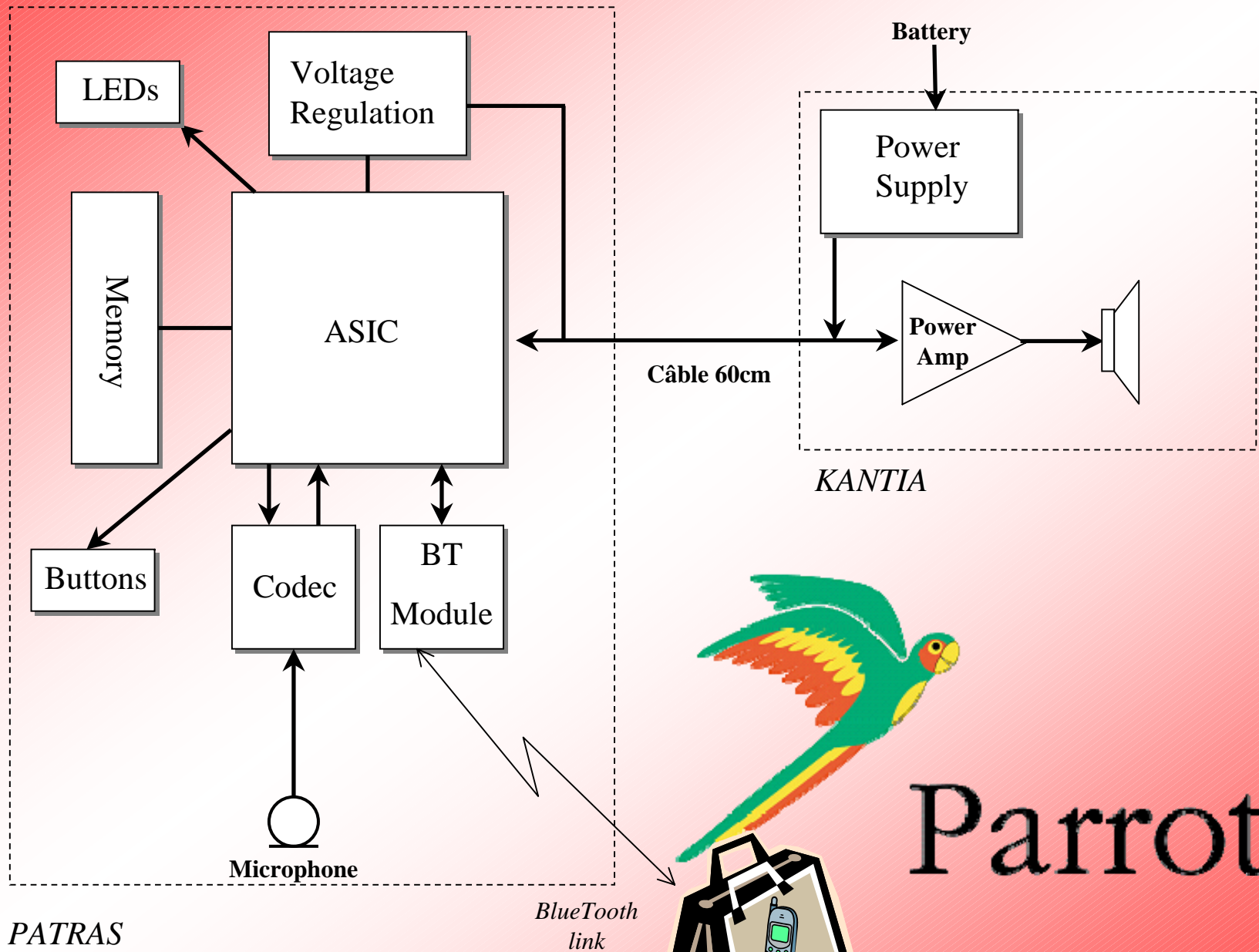
Easydrive : Block diagram
