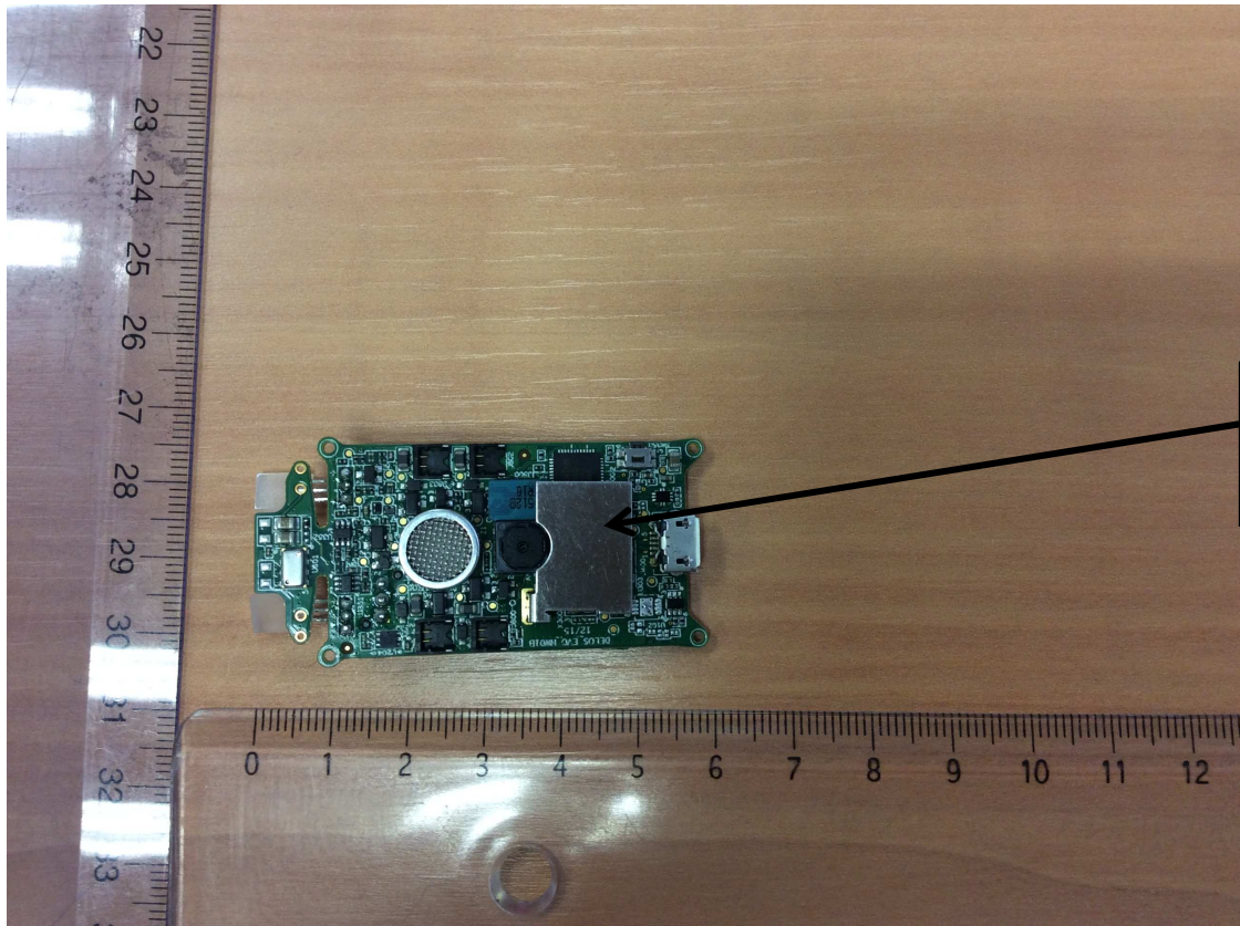
Board (Top)
