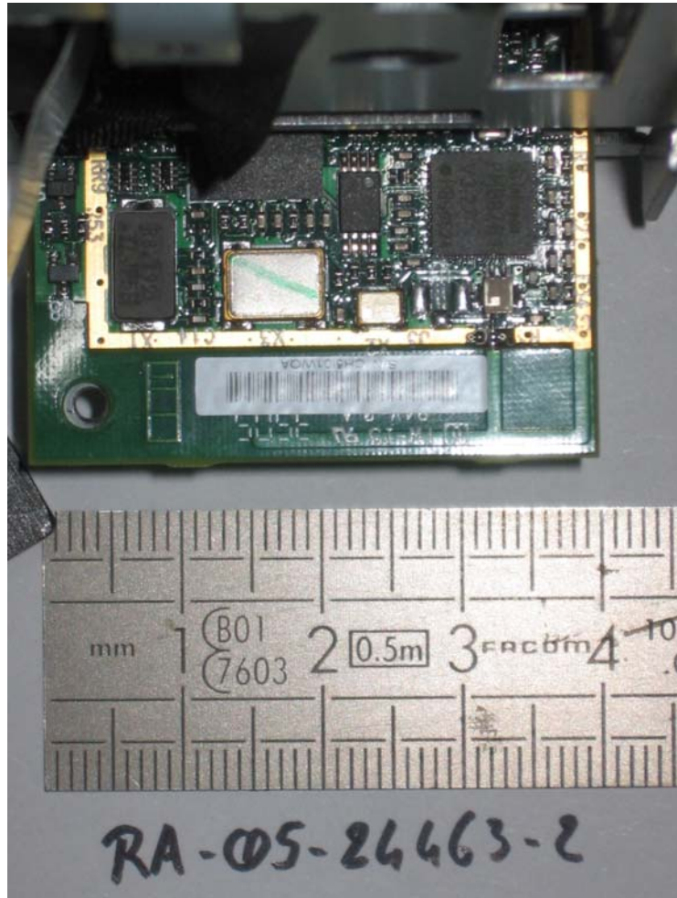
Printed circuit board Bluetooth module: face 1
