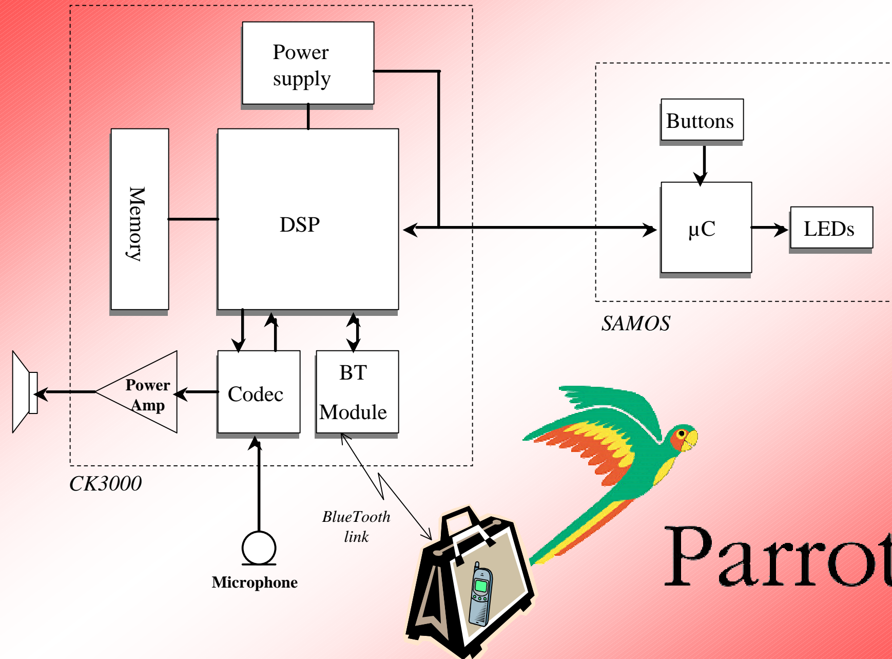
CK3000 Evolution : Block diagram
