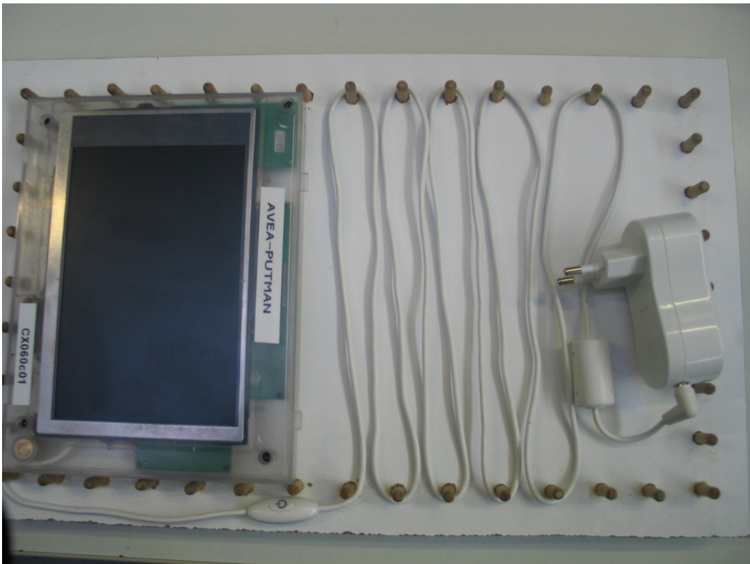
Photo 7: EUT equipped with AC/DC power supply
