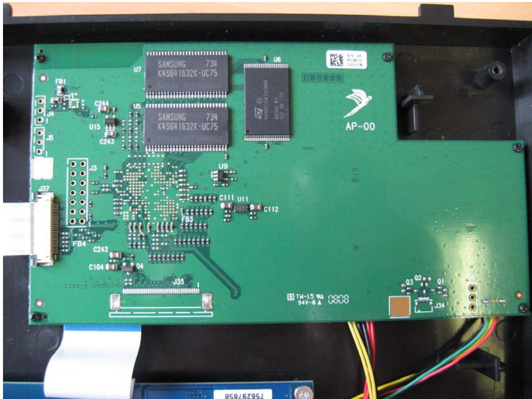
AP MOTHER BOARD (Top)
