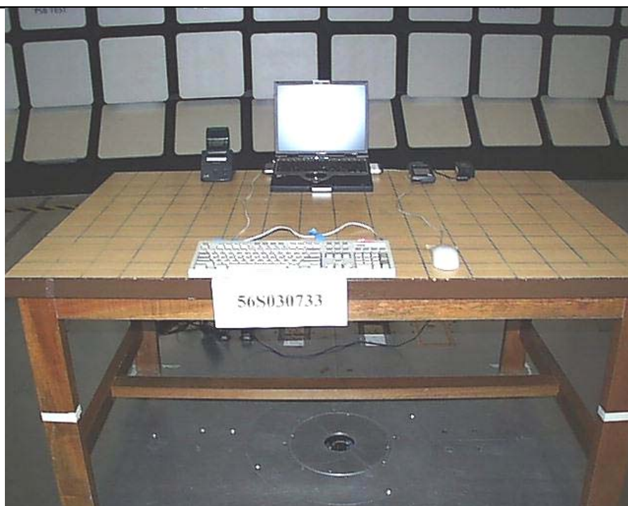
Radiated Emissions Setup (Front View)
