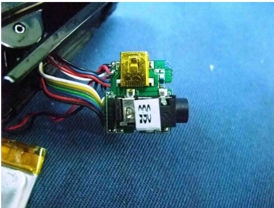
Bluetooth Headset FM PCB solder side
