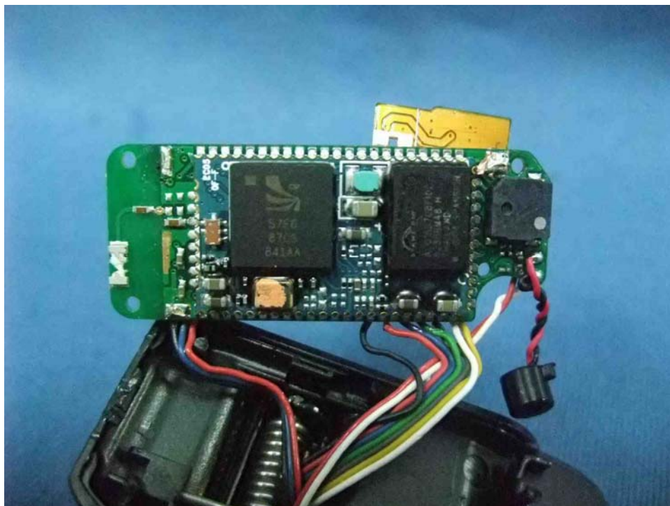
Bluetooth Headset Oscillator PCB comp side
