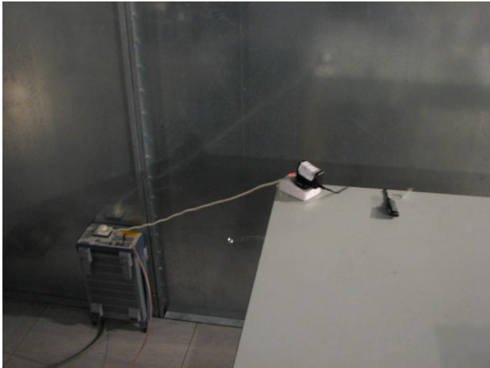
Set-up for AC wireline conducted emissions
