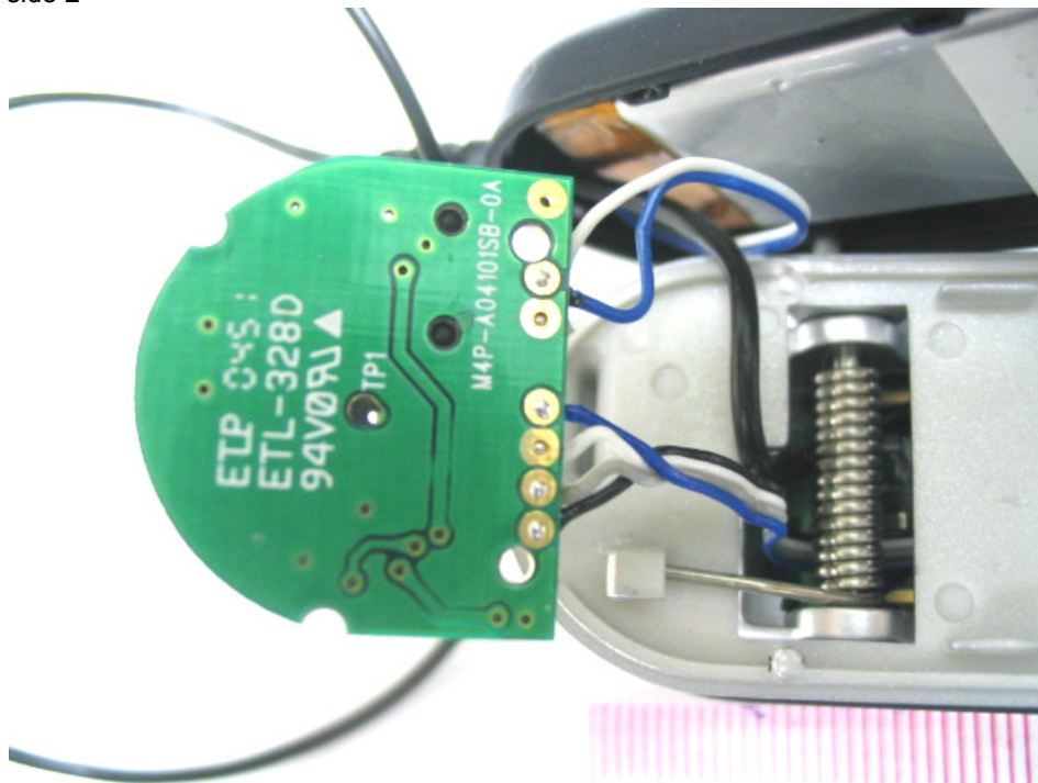
1.2.4 Rear side 2
