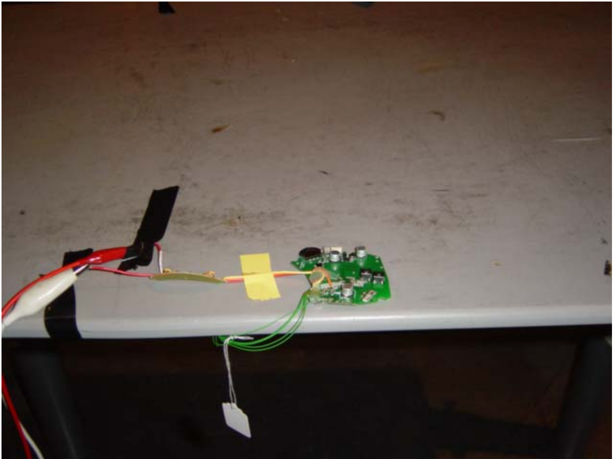
Set-up for Radiation Emission (Transceiver)
