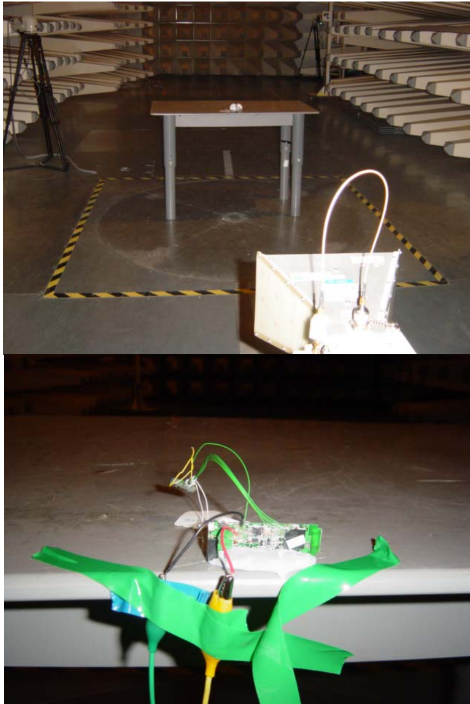
Set-up for Spurious Emission (Transceiver)
