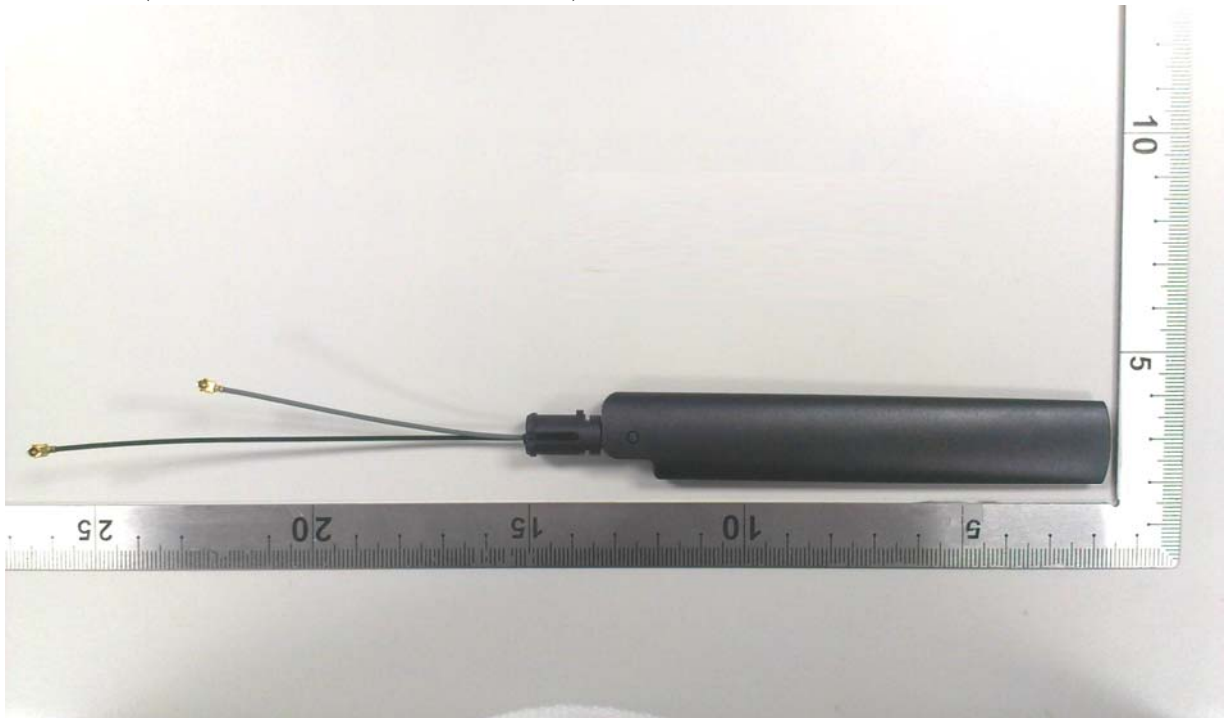
(4) EUT Photo (Ant2-Master Wave / 98619PIPF014)
