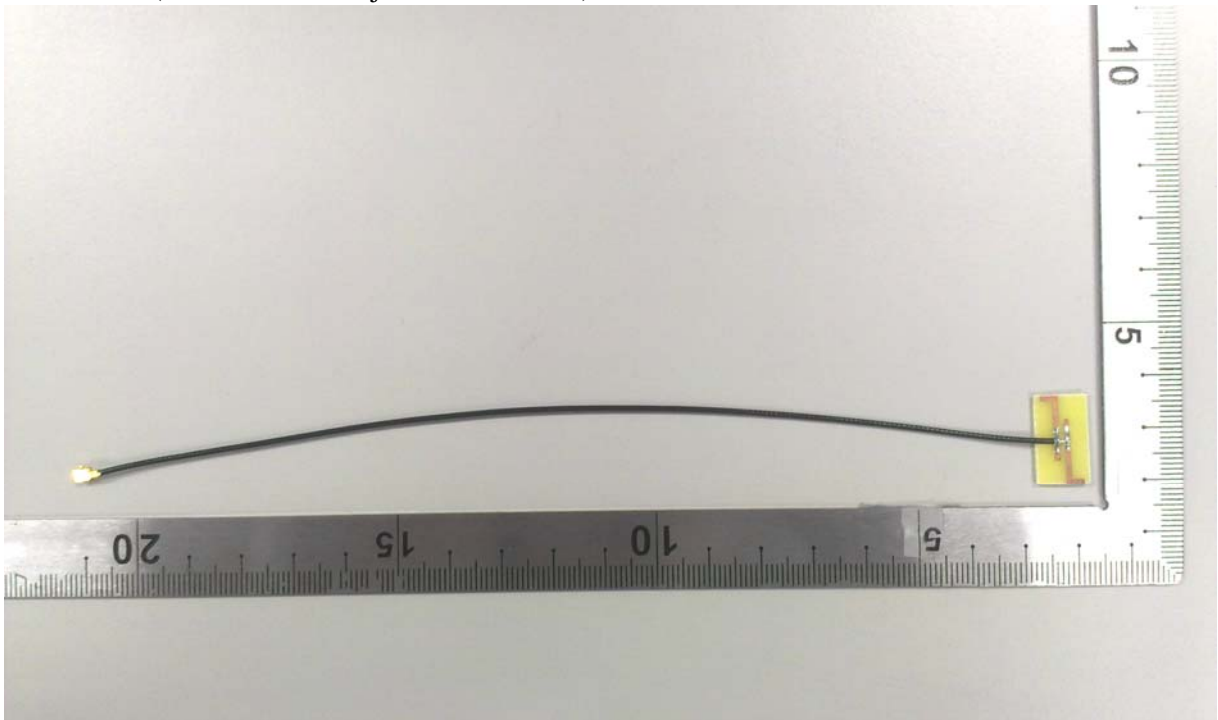
(12) EUT Photo (Ant10-Taiwan Anjie / AP11I-00003)
