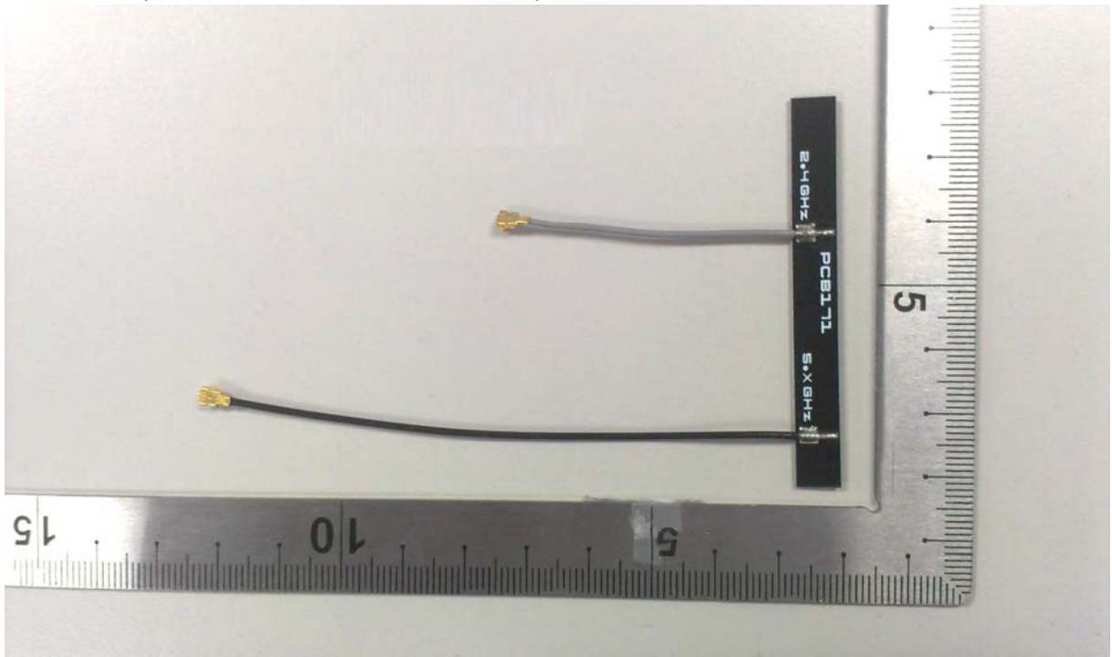
(10) EUT Photo (Ant8-Aristotle-RFA / 52-P171-TF-1)
