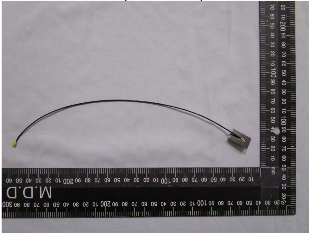
Antenna(AJWP1J-B0017) Pic 1
