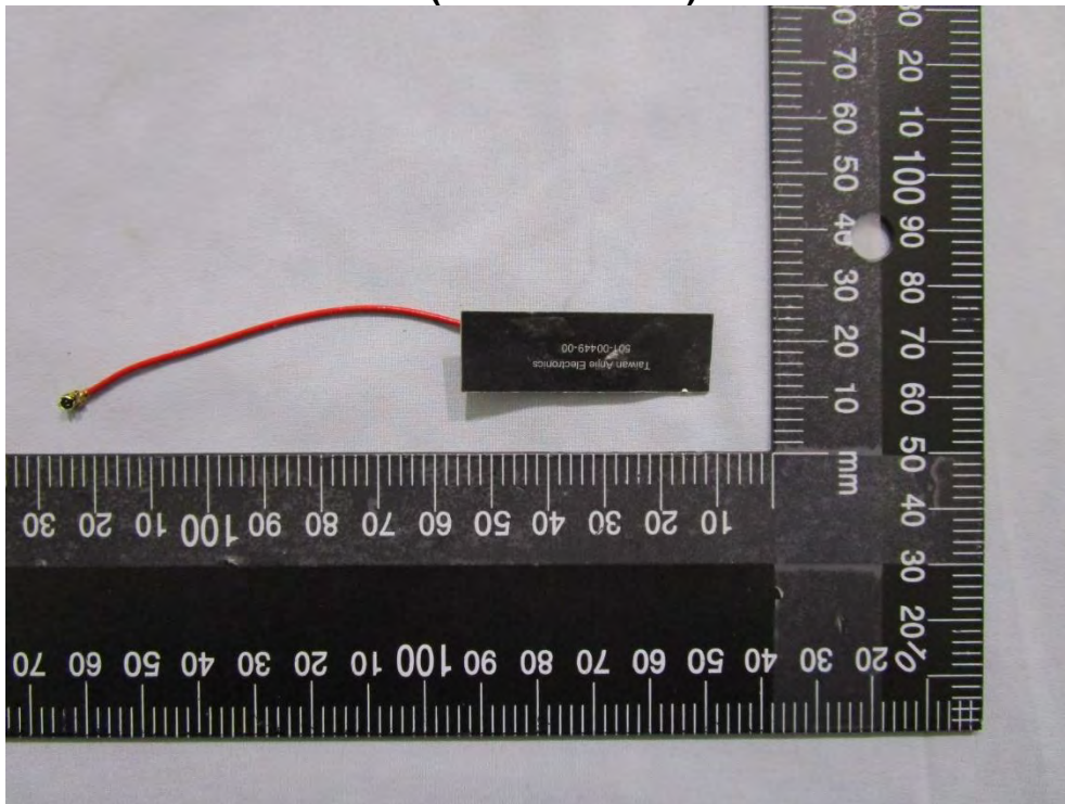
Antenna(AJDP1J-R0003) Pic 2
