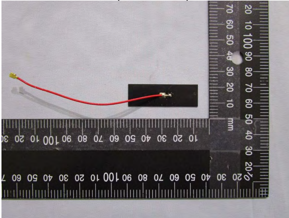
Antenna(AJDP1J-R0003) Pic 1
