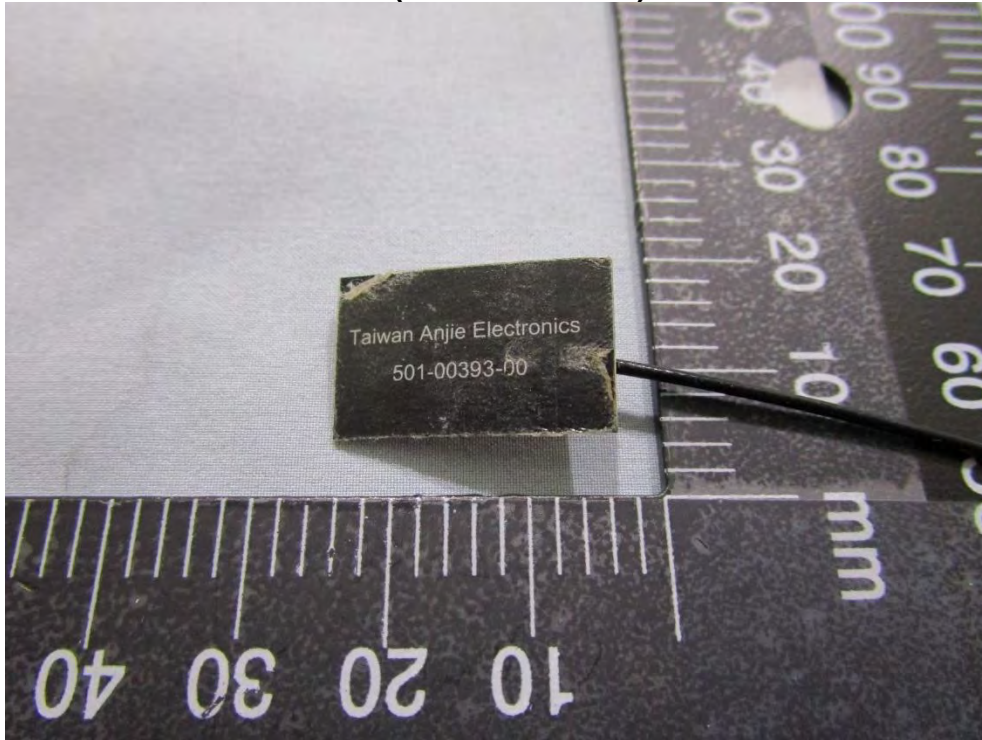
Antenna(AJWP1J-B0017) Pic 3
