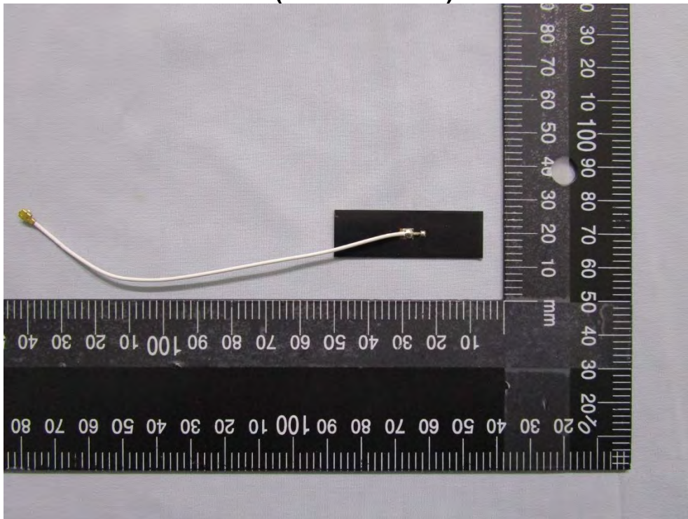
Antenna(AJDP1J-W0059) Pic 2
