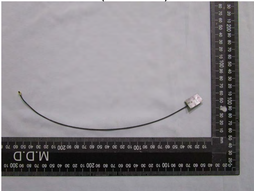
Antenna(AJWP1J-B0017) Pic 2
