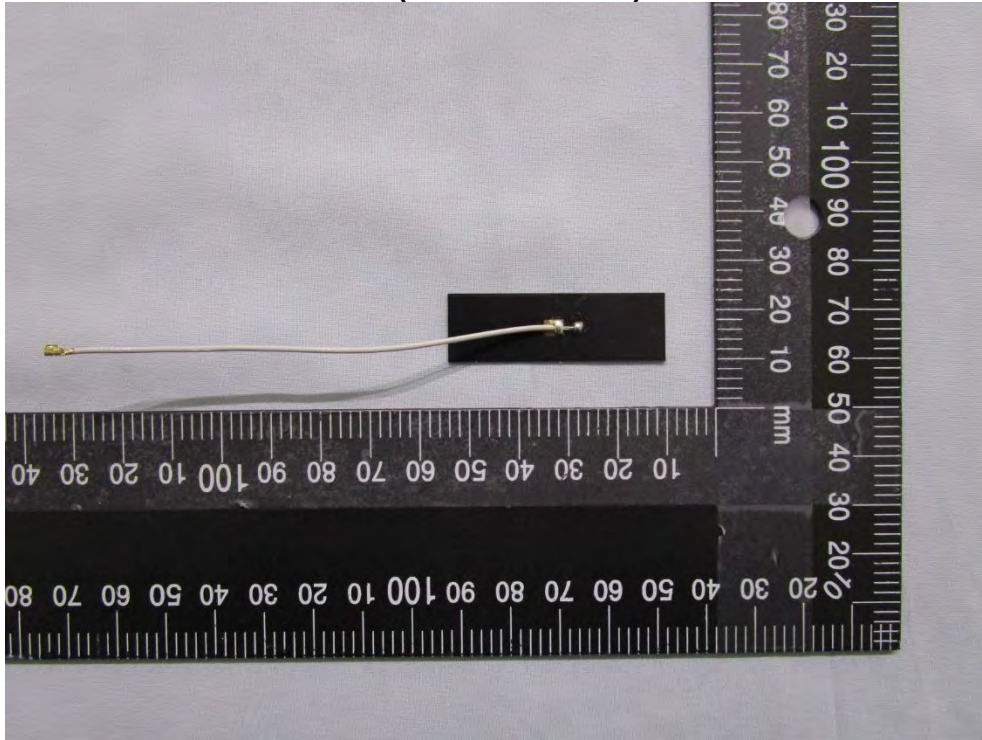
Antenna(AJDP1J-C0050) Pic 1
