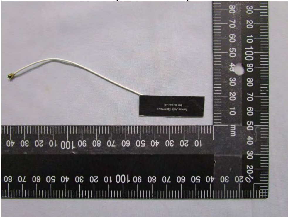
Antenna(AJDP1J-W0059) Pic 1
