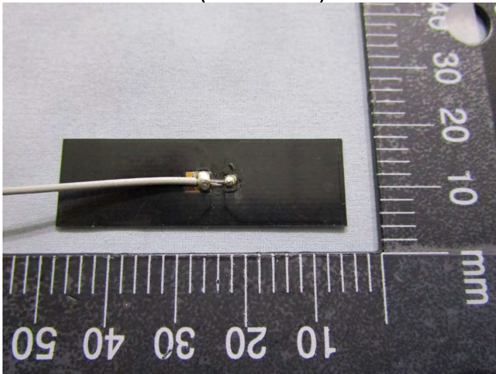
Antenna(AJDP1J-C0050) Pic 4
