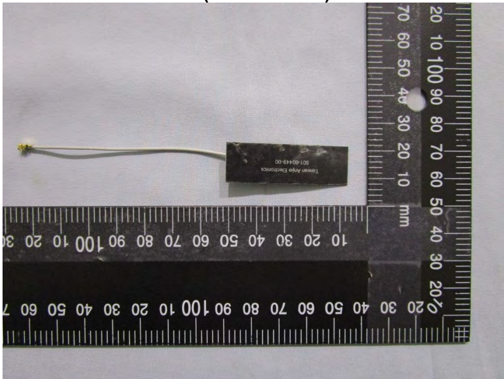
Antenna(AJDP1J-C0050) Pic 2
