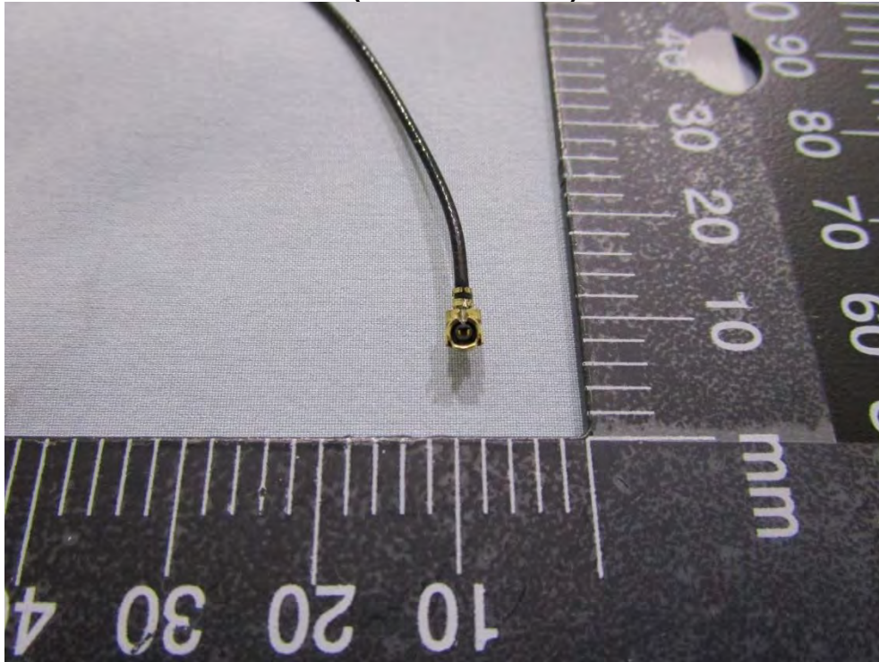
Antenna(AJWP1J-B0017) Pic 5
