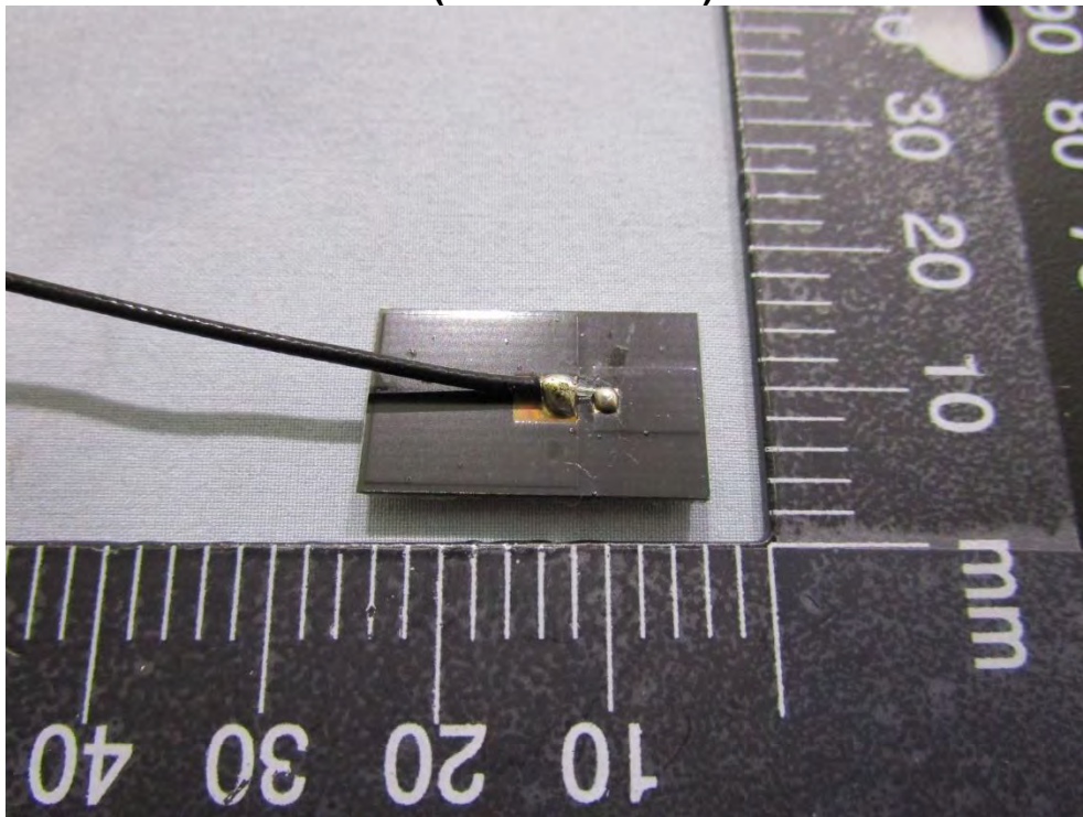
Antenna(AJWP1J-B0017) Pic 4
