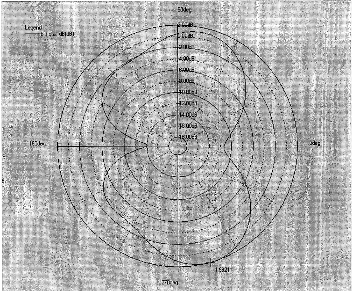
[96] 1D view / Frequency=2450.00MHz
