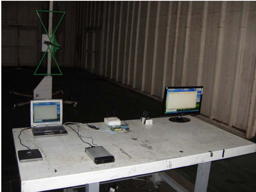
Back View of Radiated Test (Dipole)
