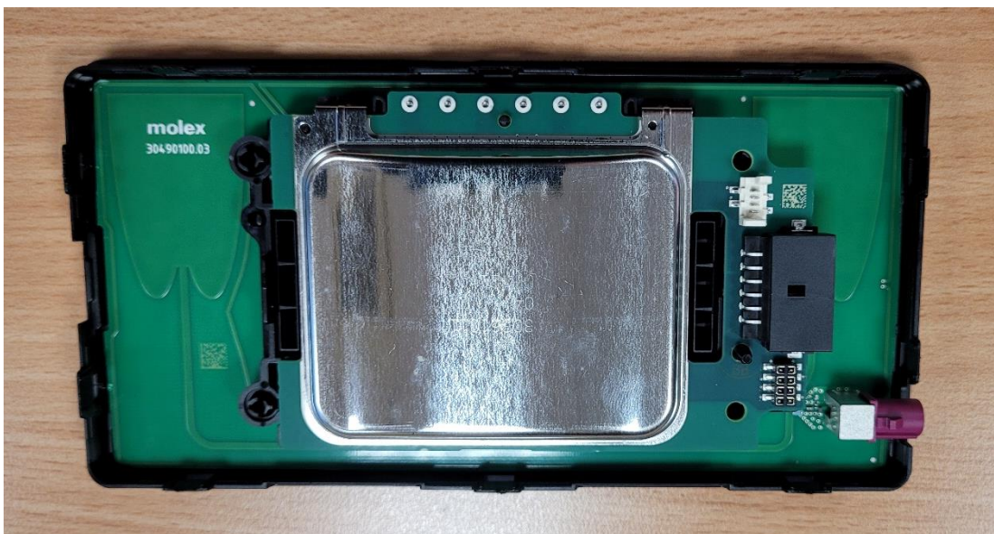
Antenna Board with Main Board and Shielding
