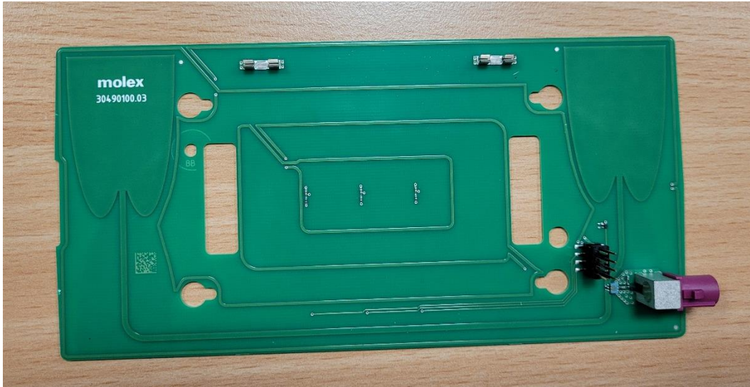
Antenna board with cellular coupler / connector
