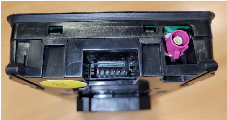
Short side view 2 with System Connector and FAKRA Connector
