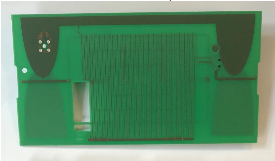
Antenna board with NFC and cellular coupler / connector
