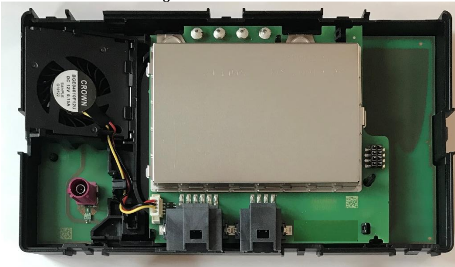
Main board with shielding
