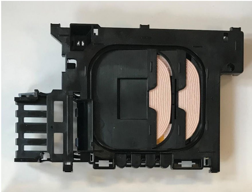
Coil board
