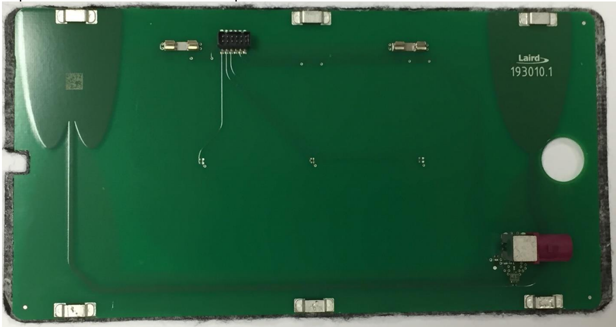
Top view of antenna board with compensator connector
