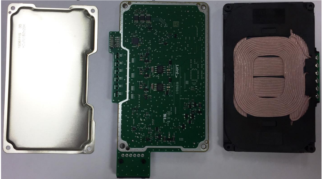
Main board with cooling element and shielding
