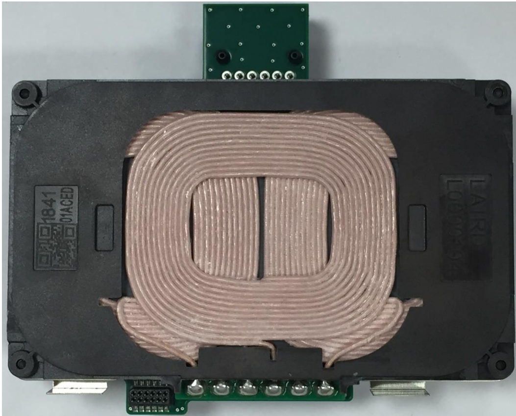
Coil module
