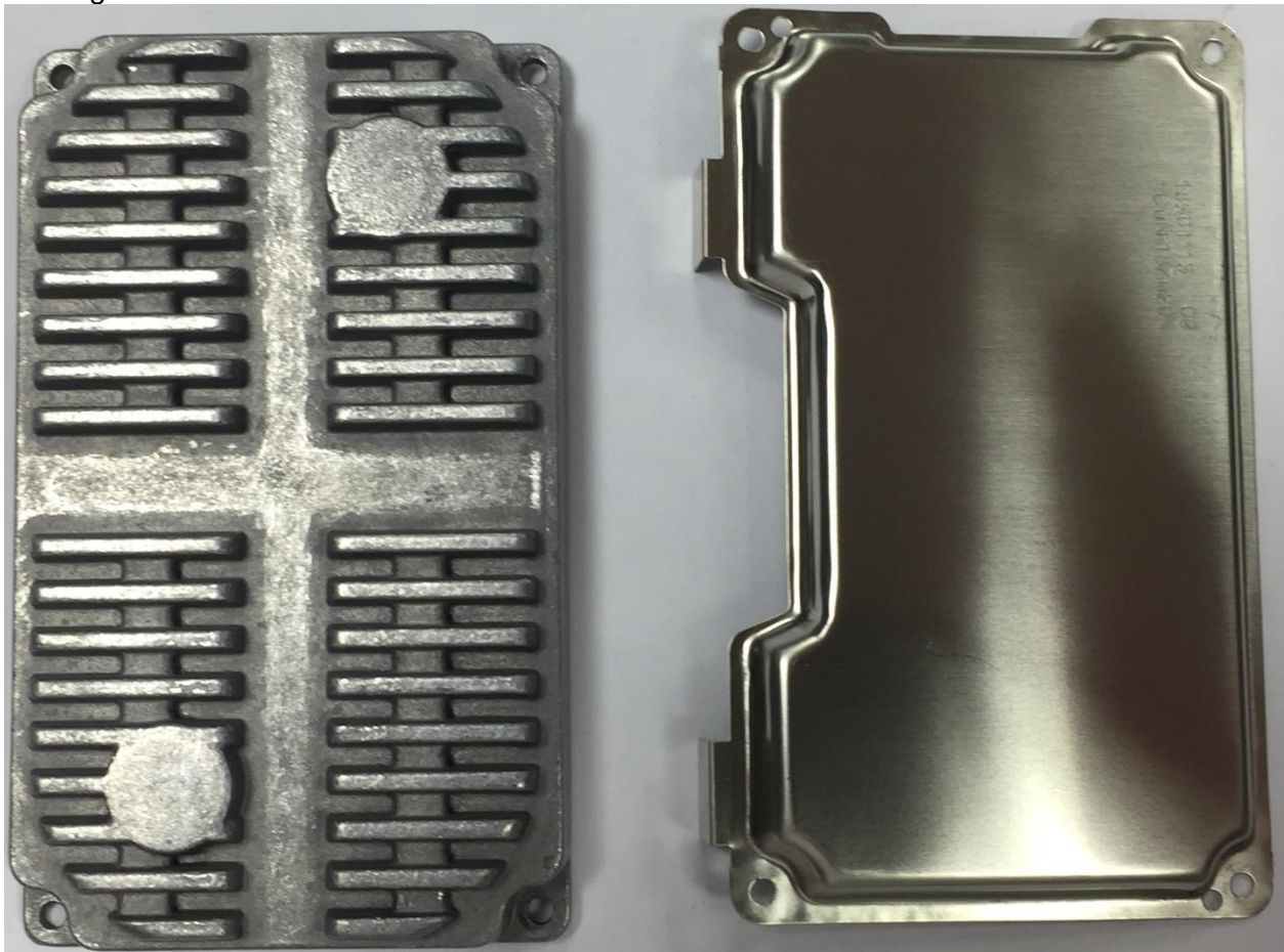
Cooling element
