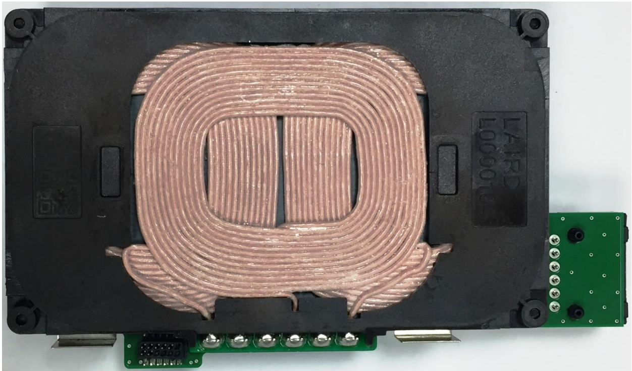
Coil module
