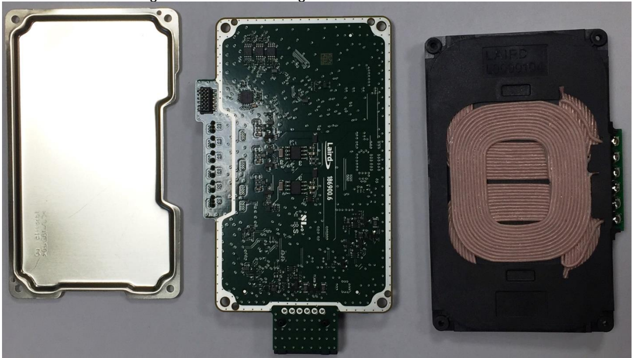
Main board with cooling element and shielding
