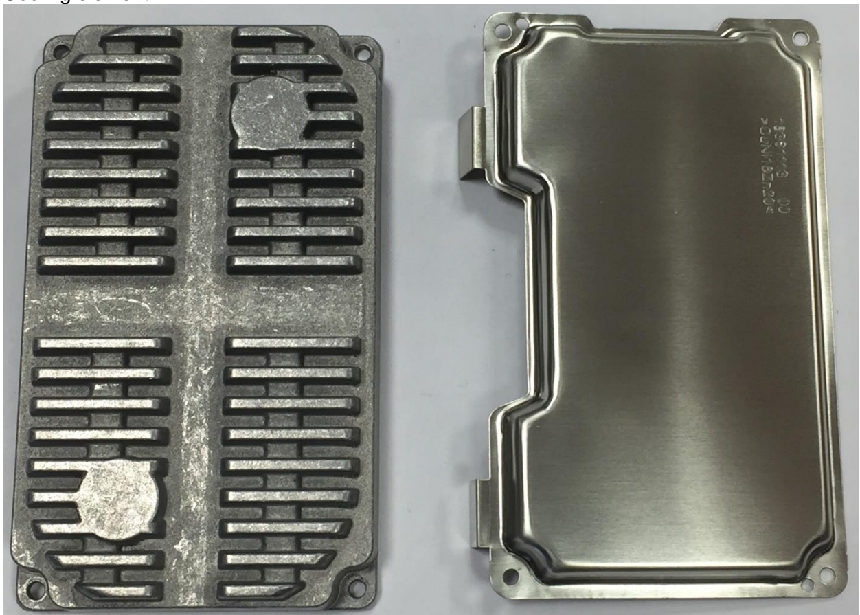
Cooling element
