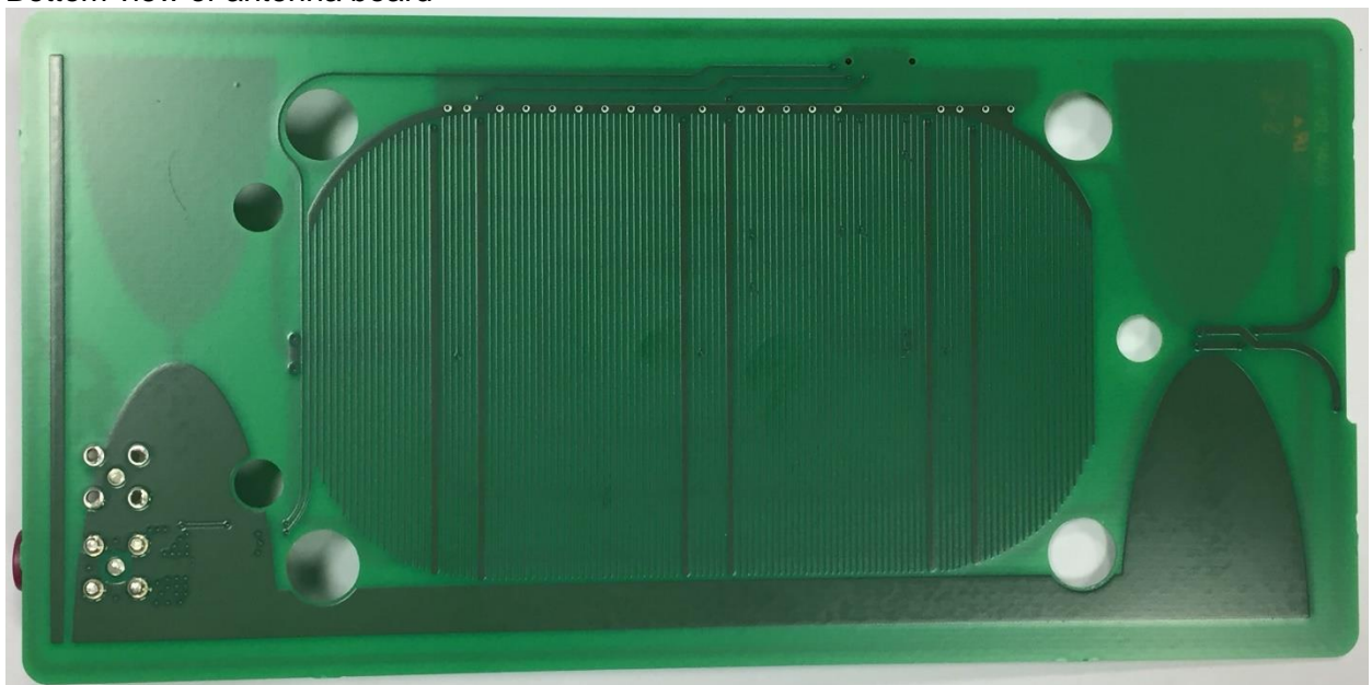
Bottom view of antenna board
