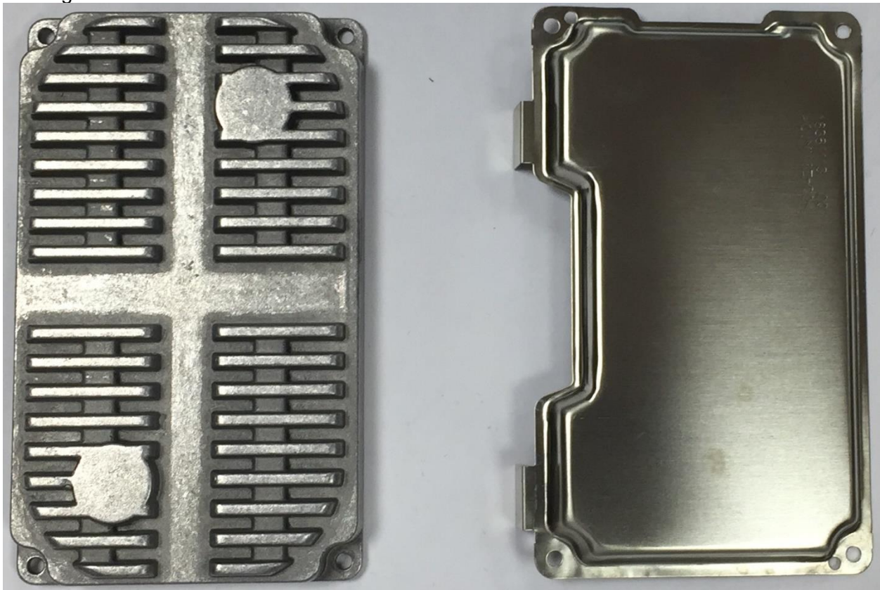
Cooling element
