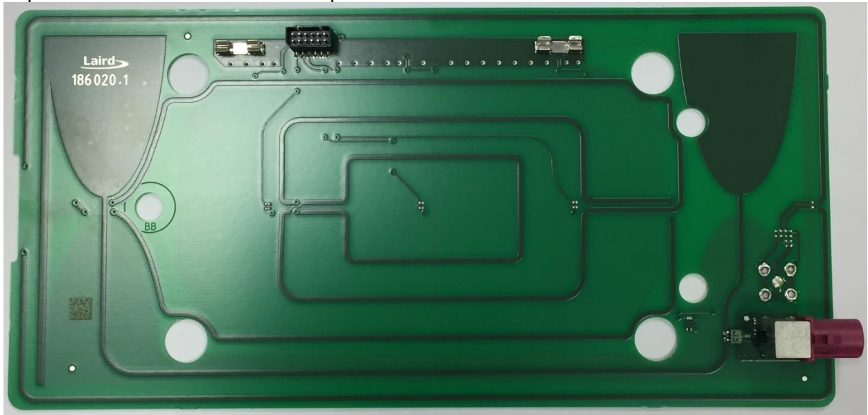
Top view of antenna board with compensor connector
