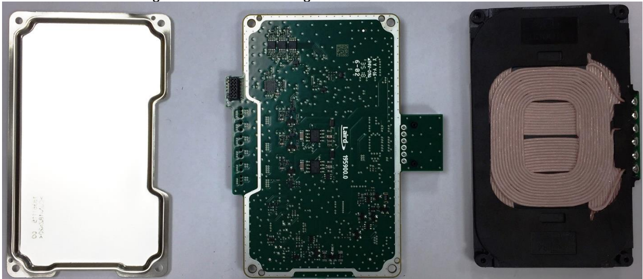
Main board with cooling element and shielding
