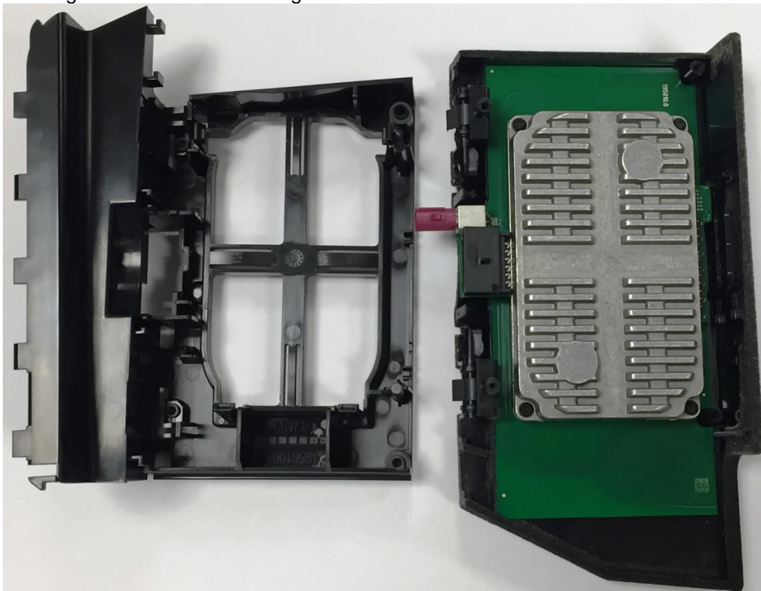
Housing bottom view with cooling element
