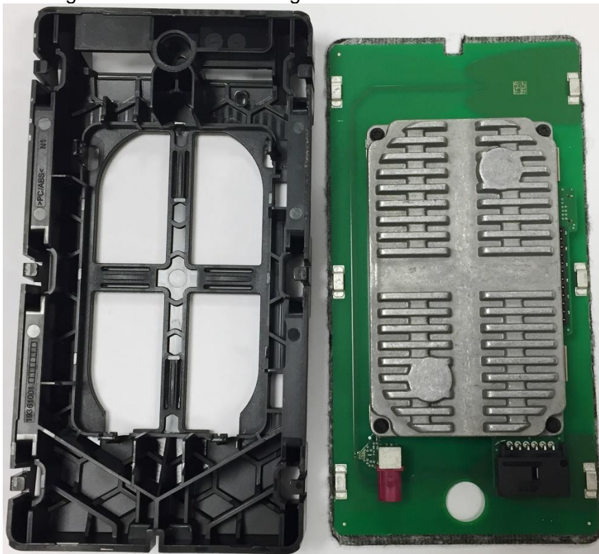
Housing bottom view with cooling element
