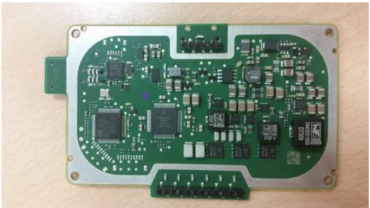
Main Board – Top & Bottom View:
