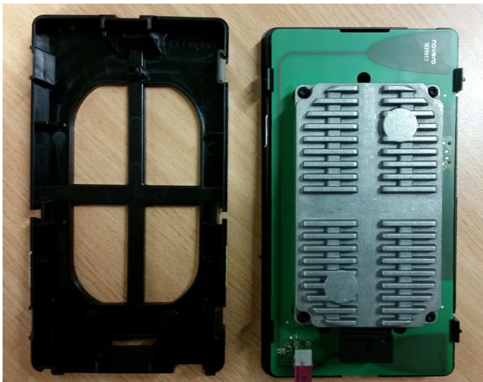
Inside view with PWBs and cooling element
