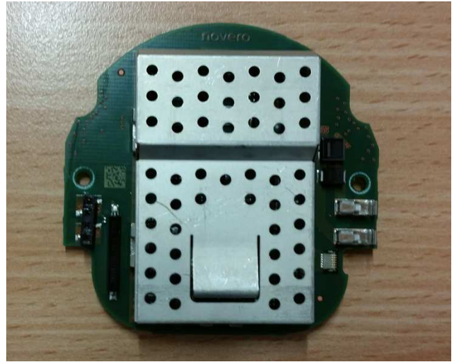
Main Board (Top view) without and with shielding
