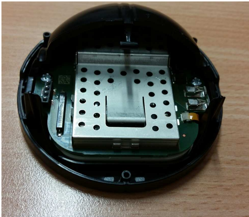
Inner view with PWB
