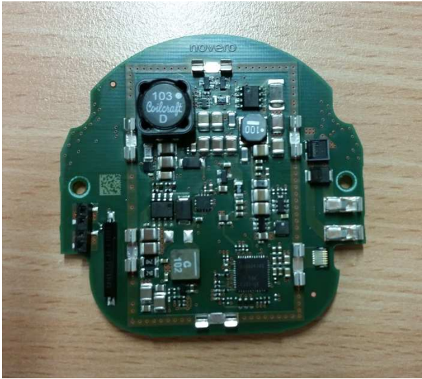
Main Board (Top view) without and with shielding
