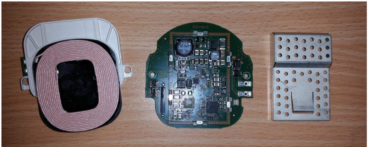
Coilmodule and Mainboard without shielding
