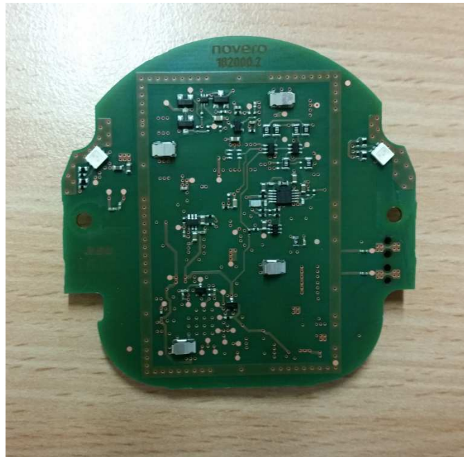
Main Board (Bottom view)
