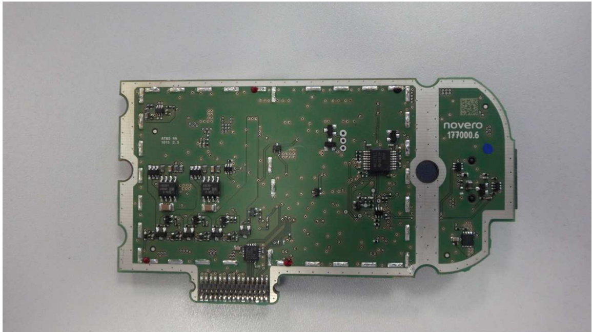
Bottom view main PCB without shielding
