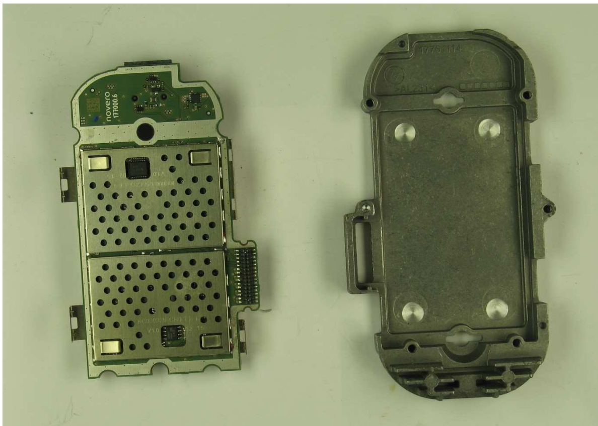
Bottom view main PCB with shielding
