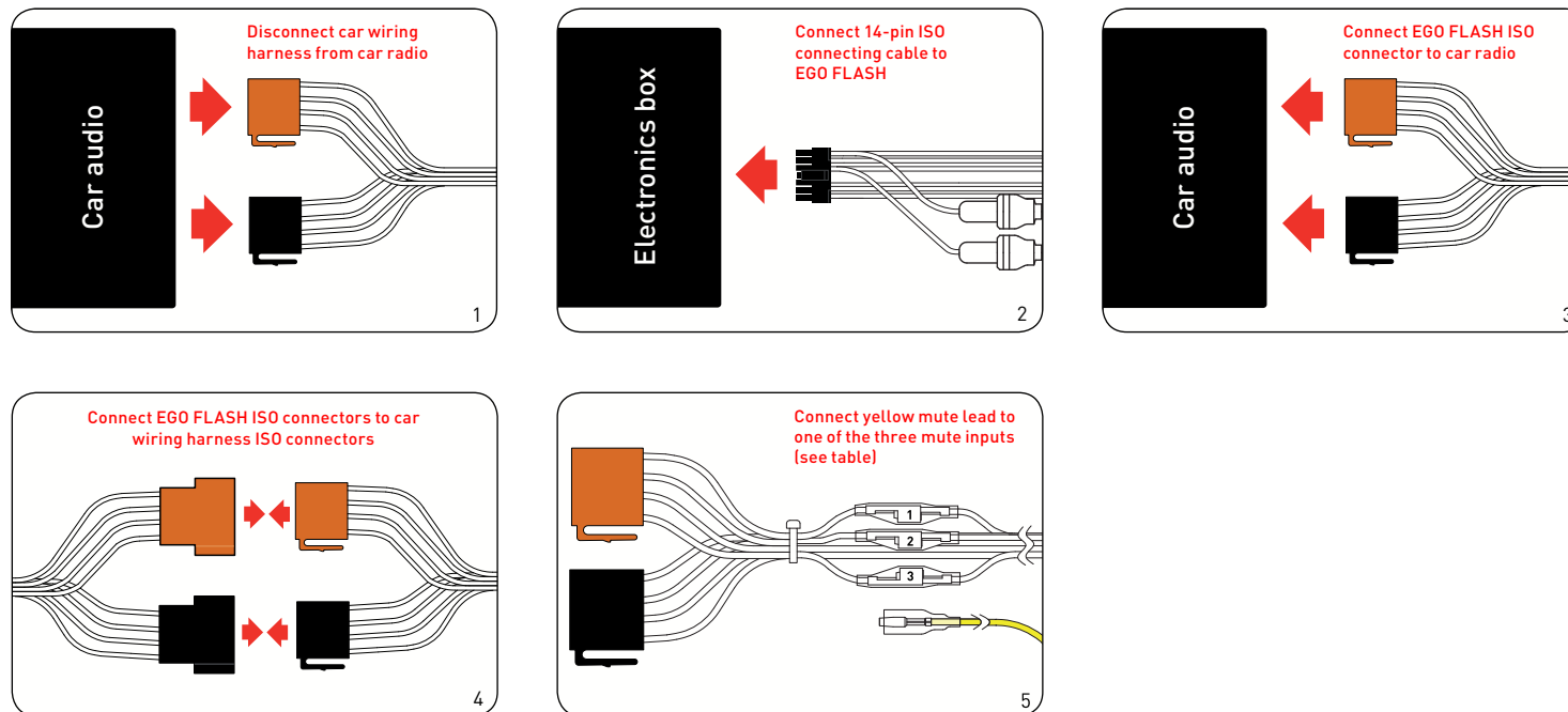
Fig. 07: Installation procedure
