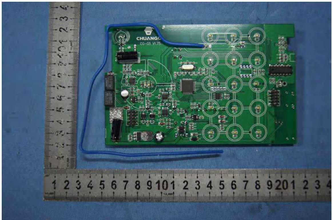
Receiving 315.8599MHz signal antenna
