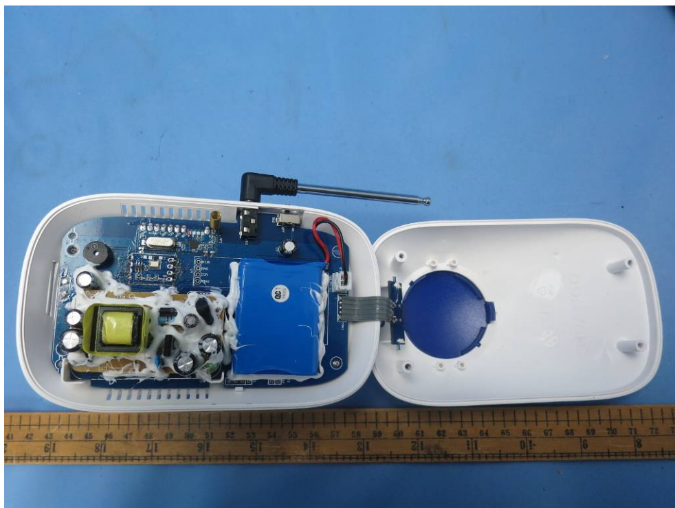
Internal Photo
