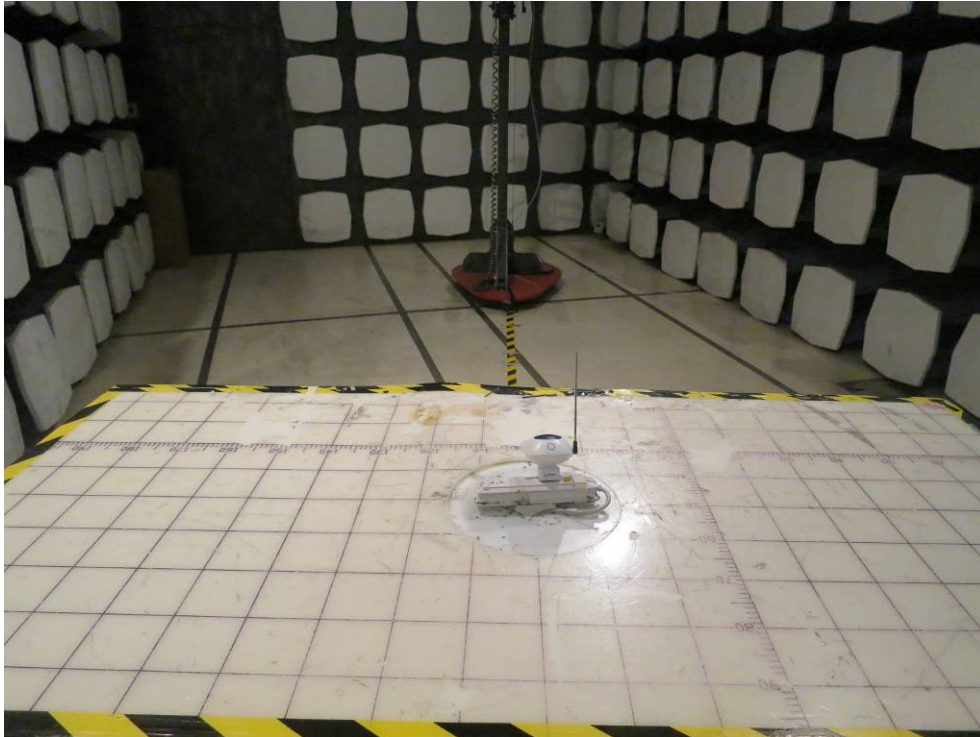
Test Setup Photo –Radiated Emission Below 1G
