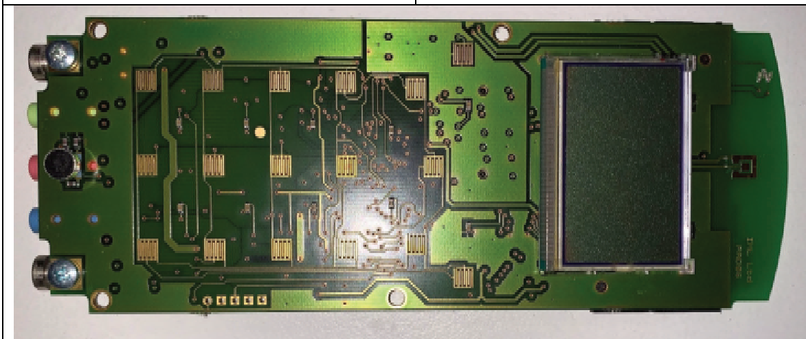
RF module and card holder removed
