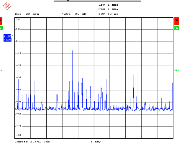
Hop rate-2441MHz
