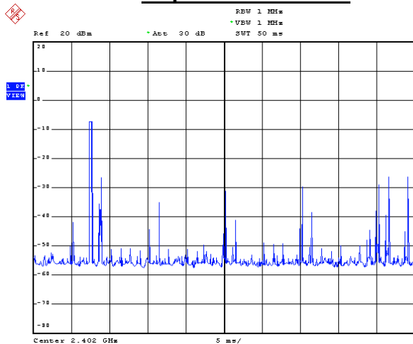
Hop rate-2402MHz
