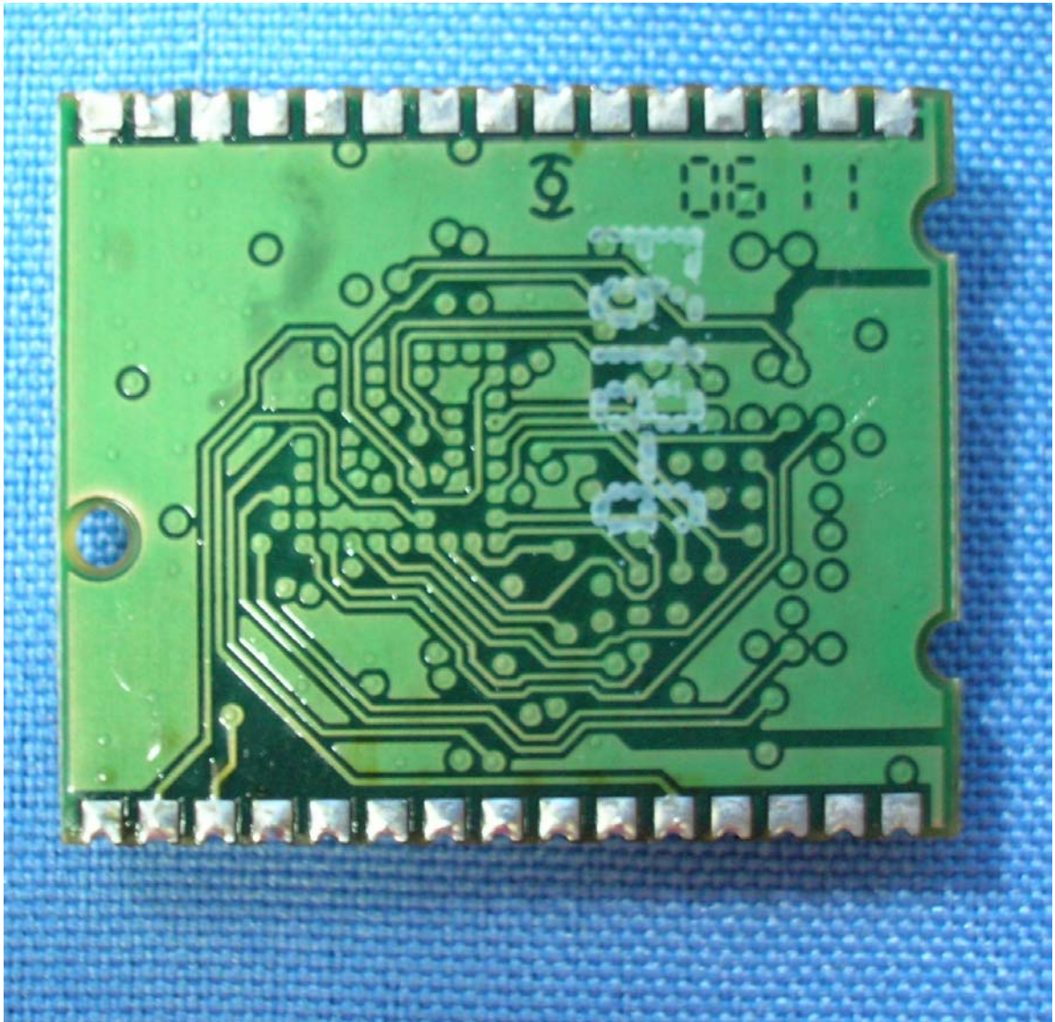
(22) EUT Photo
